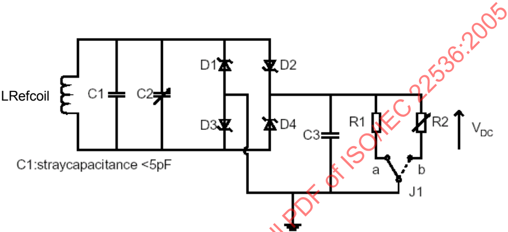
Figure C.1 — Circuit diagram for reference device
