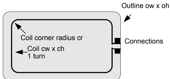
Figure 1 — Calibration coil
