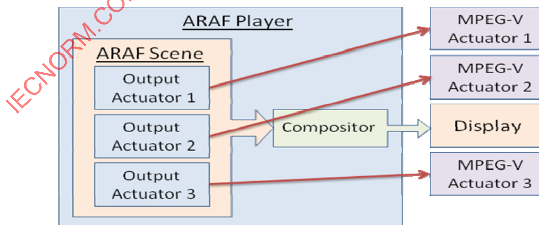
Figure 4 — Diagram of the architecture for commanding MPEG-V actuators
