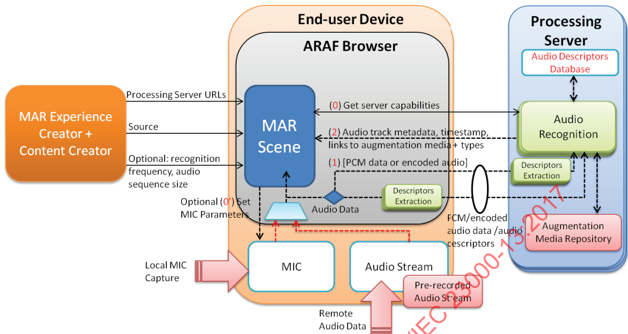
Figure 11 — Remote audio recognition
