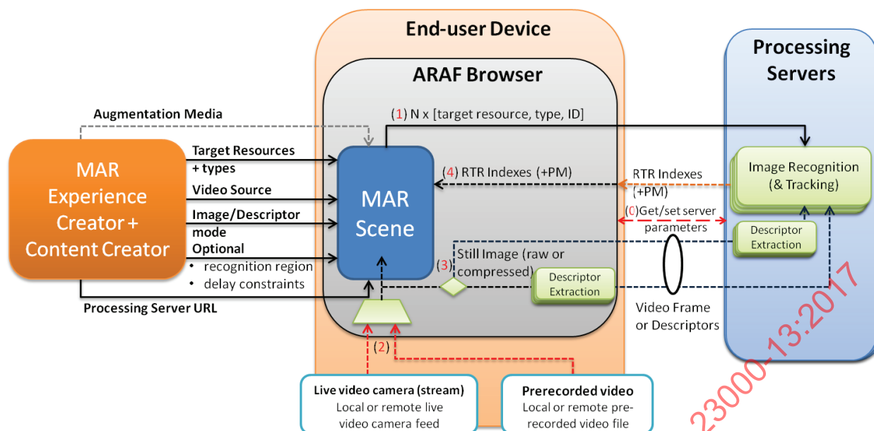
Figure 5 — Remote image recognition registration proxy
