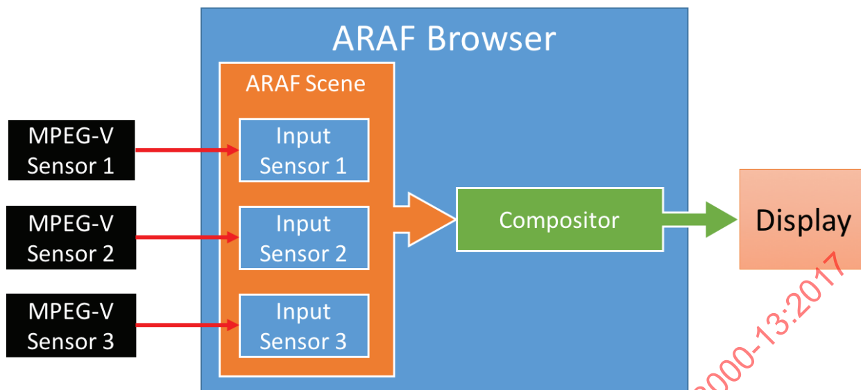
Figure 12 — Diagram of the architecture for accessing MPEG-V sensor data
