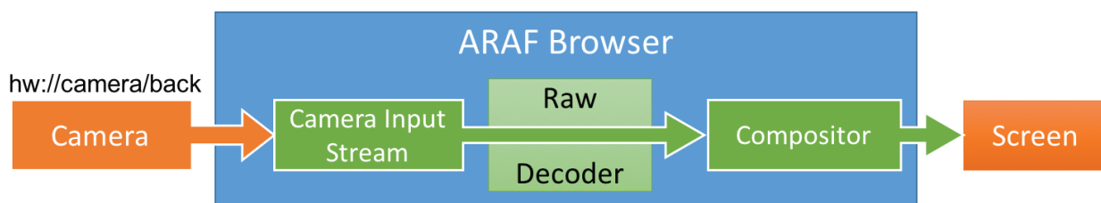
Figure 13 — Diagram of the architecture for accessing the camera frames
