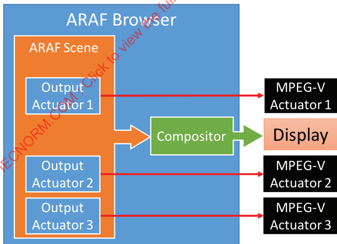
Figure 144 — Diagram of the architecture for commanding MPEG-V actuators
