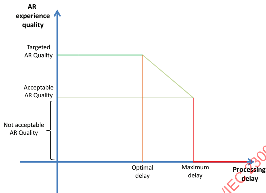
Figure 6 — RemImgProxy: AR quality vs. processing delay
