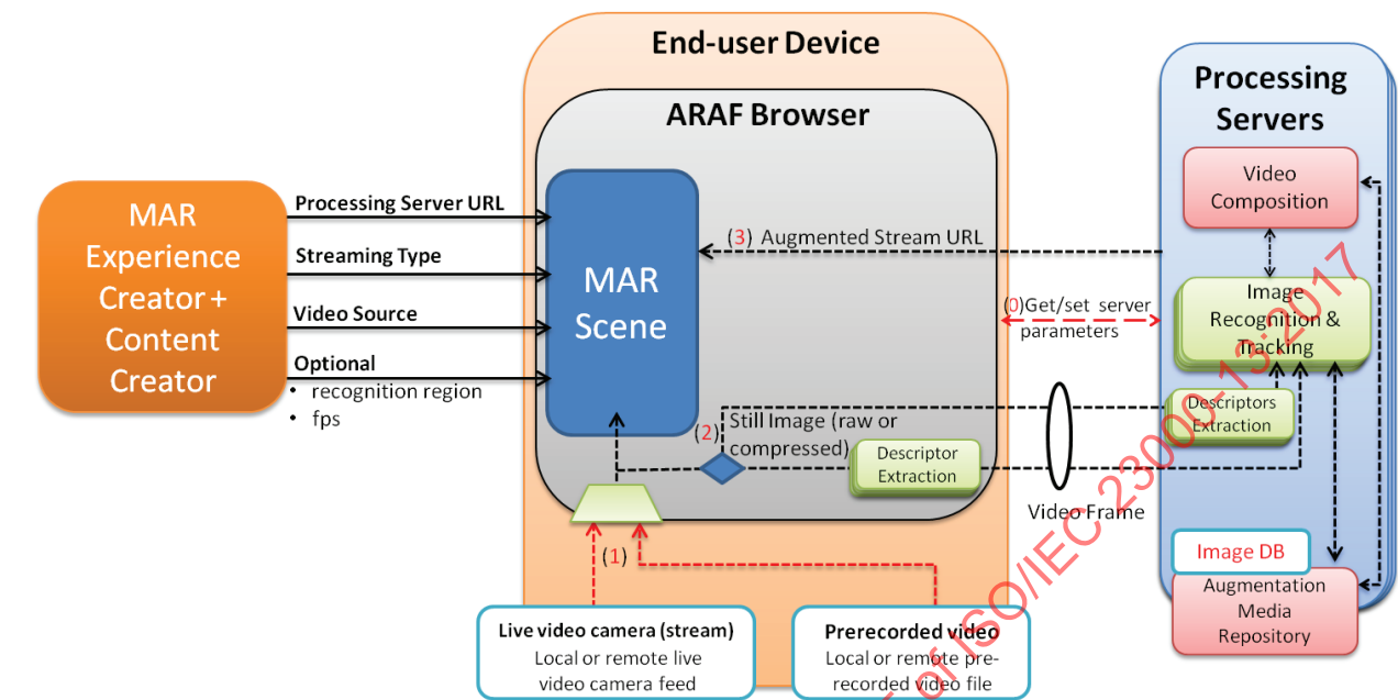
Figure 9 — Remote image recognition registration composition
