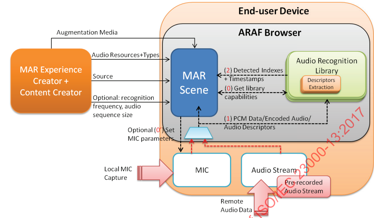
Figure 10 — Local audio recognition
