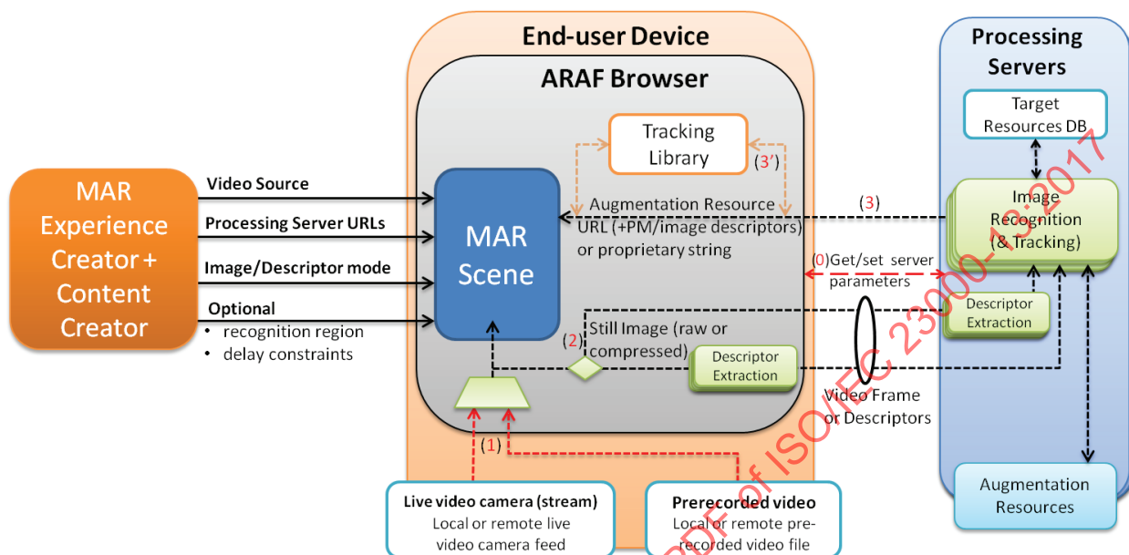
Figure 7 — Remote image recognition registration server
