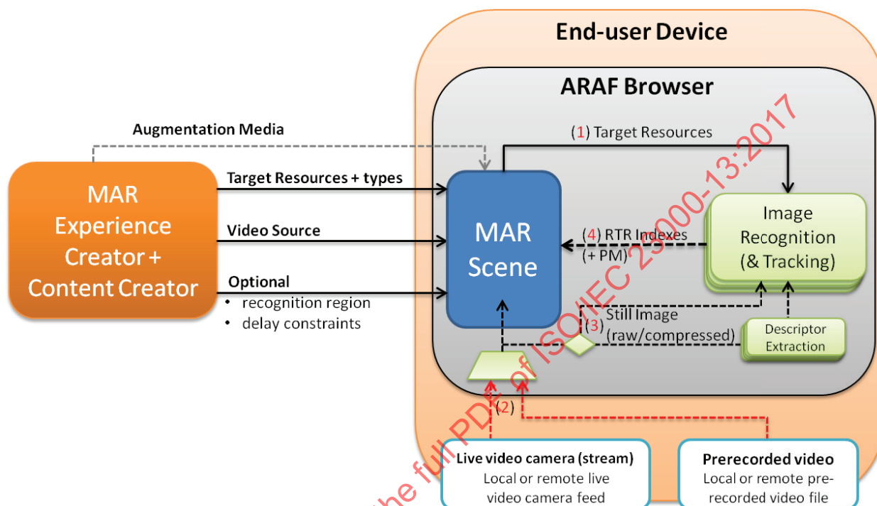
Figure 3 — Local image recognition registration
