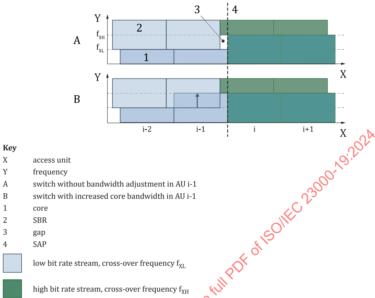
Figure 16 — Illustration of core bandwidth adjustment for HE-AAC switching points
