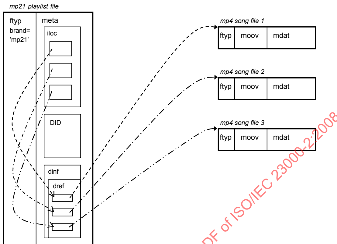
Figure 11 — Linkage of mp21 playlist file referencing external mp4 song files
