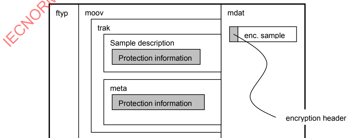
Figure 19 — Protection information inside an mp4 file and encrypted samples
