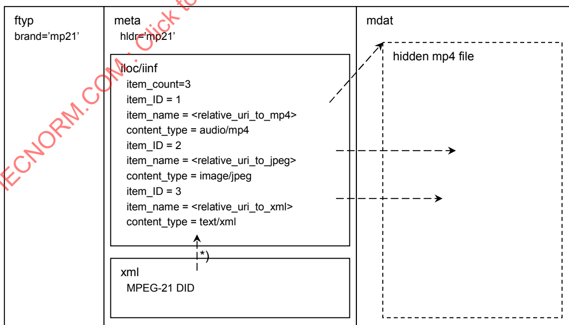
Figure 9 — Example of file structure for mp21 file containing one hidden mp4 song file
