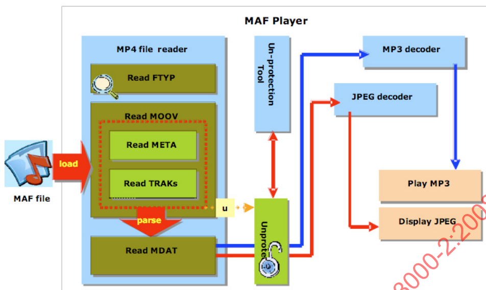
Figure 20 — Software architecture of the Music Player MAF application
