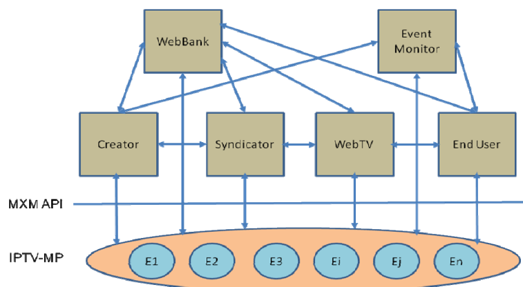
Figure J.1 — IPTV-MP implemented using the MXM standard
