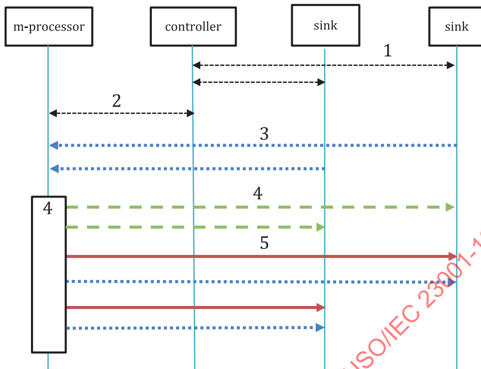
Figure 17 — Spatial orchestration at the sink side
