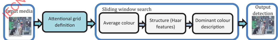
Figure 24 — DROP search process
