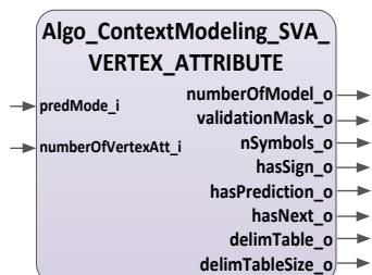
ContextModeling_SVA_Vertex_Attribute Process Schematic (FSM):
