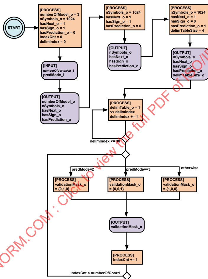
ContextModeling_SVA_Vertex_Attribute Process Schematic (FSM):
