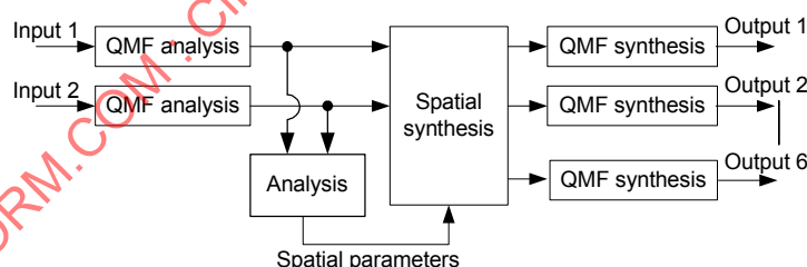
Figure 18 — Overview of parameter-less SAC extension
