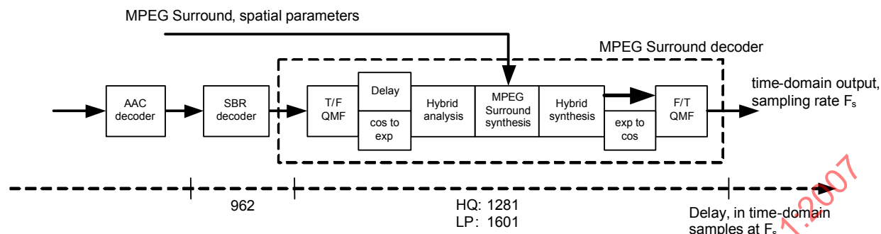
Figure 11 — Delay when connecting MPEG Surround in the time-domain for arbitrary core codec (including HE-AAC)
