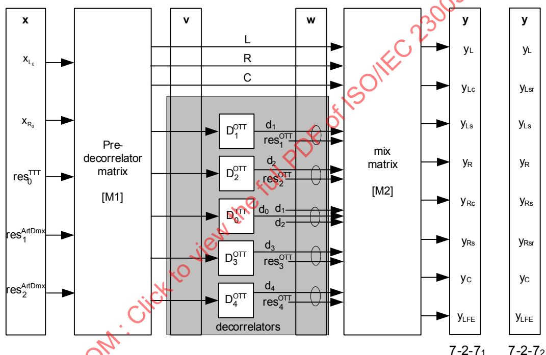
Figure 27 — Matrix view of the spatial audio processing for the 7-2-7 configurations
