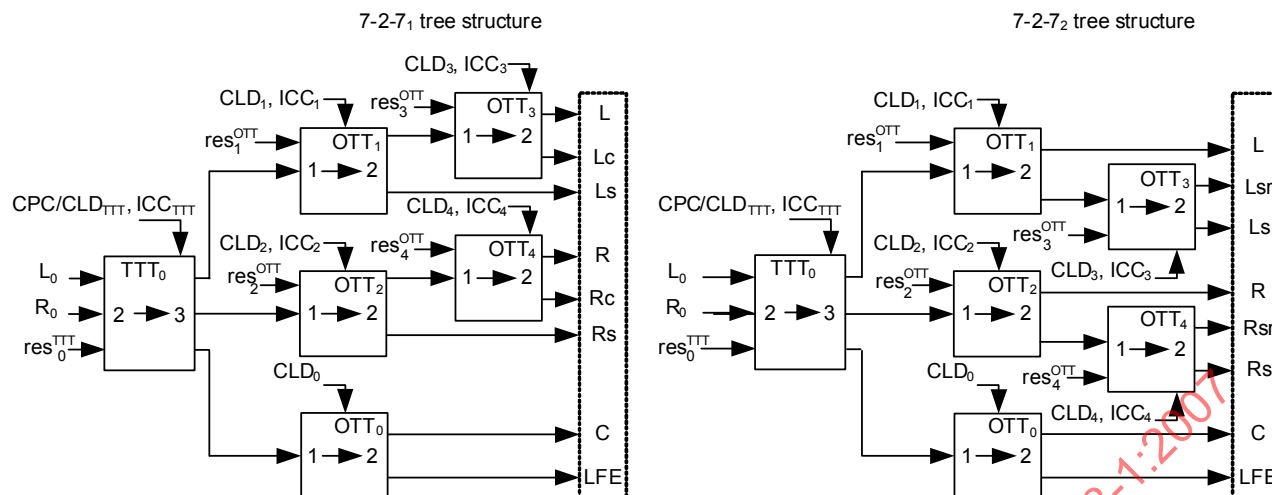
Figure 28 — Tree structure view of the spatial audio processing for the 7-2-7 configurations
