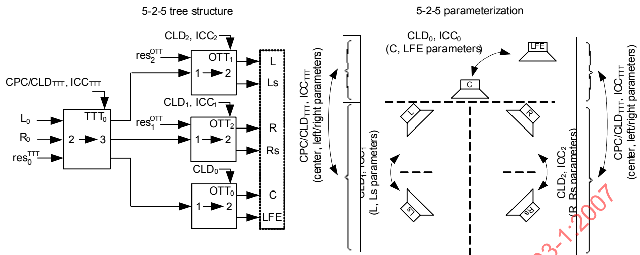
Figure 26 — Tree structure and parameterization view of the spatial audio processing for the 5-2-5 configuration
