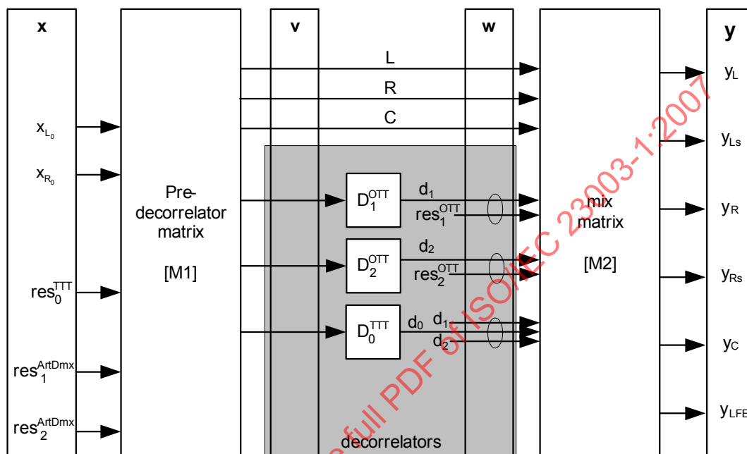
Figure 25 — Matrix view of the spatial audio processing for the 5-2-5 configuration
