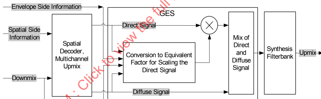
Figure 37 — Placement of the Guided Envelope Shaping tool in the decoder
