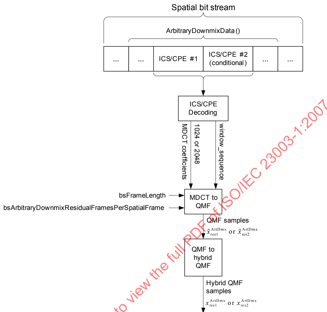
Figure 39 — Overview of artistic enhancement residual decoding process of residual decoding process.
