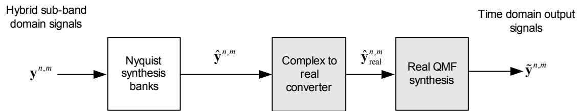
Figure 44 — Time/frequency transforms for Low Power MPEG Surround, hybrid QMF synthesis bank
