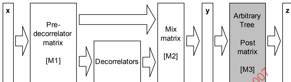
Figure 33 — Matrix view of the spatial audio processing when adding the arbitrary trees as a post process
