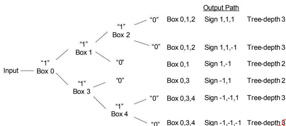
Figure 16 — Graphical representation of the relation between the tree descriptive variables, and the signaled tree.
