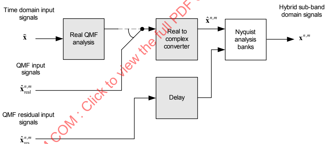
Figure 43 — Time/frequency transforms for Low Power MPEG Surround, hybrid QMF analysis bank
