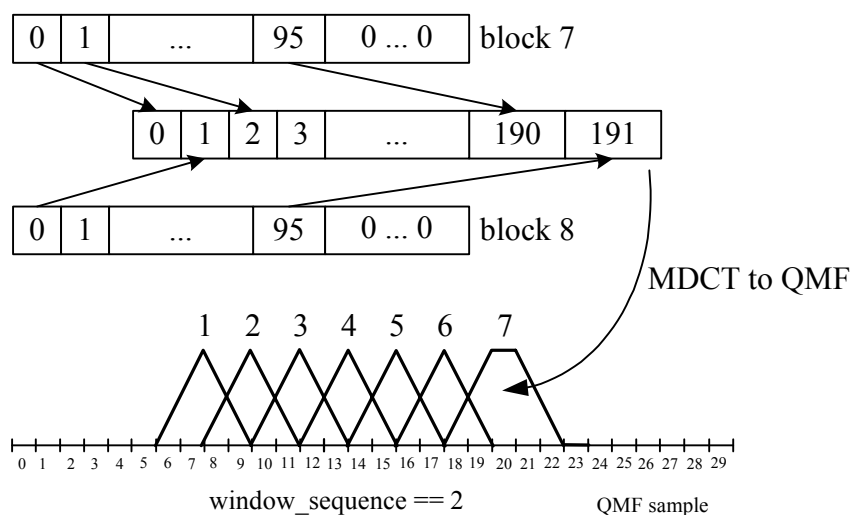
Figure 41 — Merging the MDCT coefficients from two last AAC short blocks into one set of 192 MDCT coefficients for window 7.
