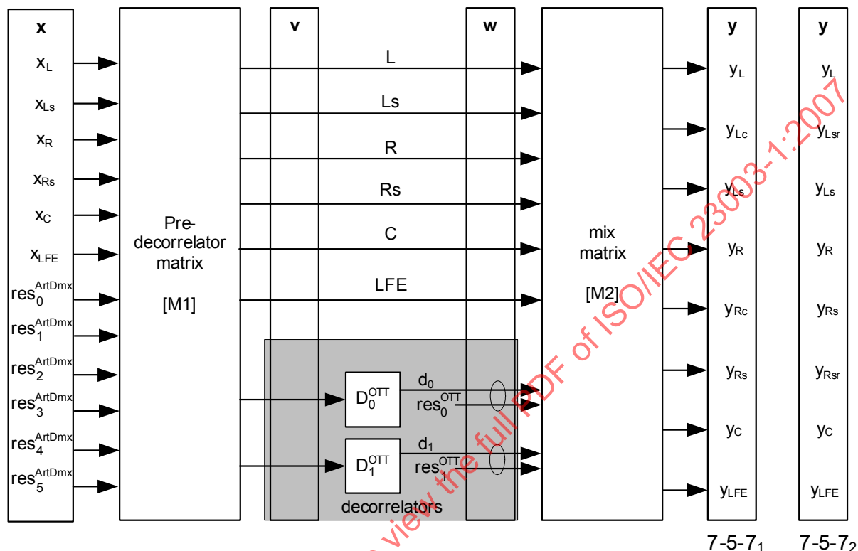
Figure 30 — Matrix view of the spatial audio processing for the 7-5-7 configurations
