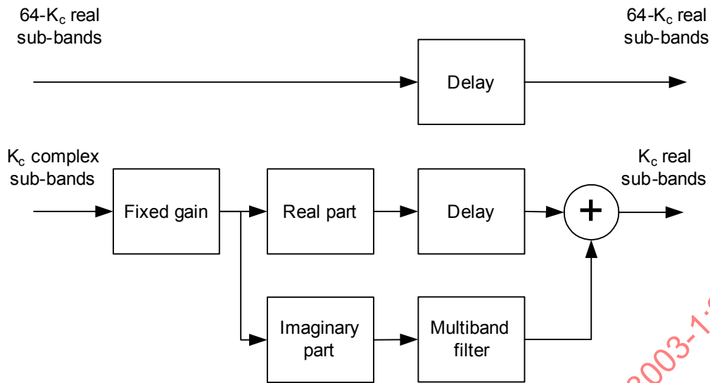
Figure 47 — Complex to real converter
