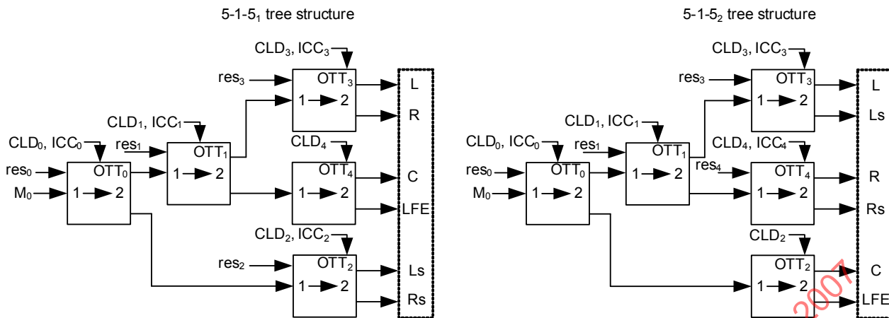
Figure 23 — Tree structure view of the spatial audio processing for the 5-1-5 configurations
