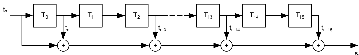
Figure 57 — The de-randomization circuit.
