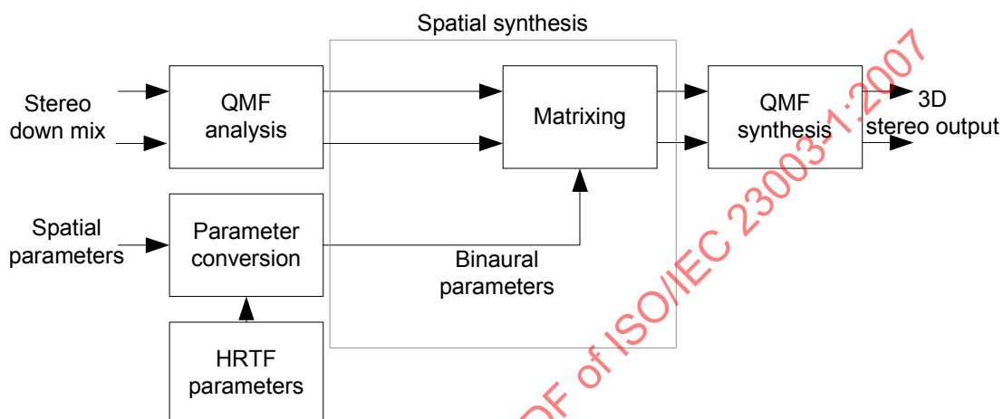
Figure 53 — 3D binaural decoder for '525' spatial configurations
