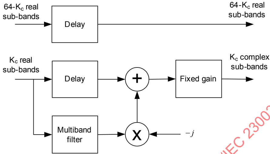
Figure 46 — Real to complex converter
