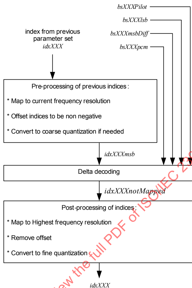
Figure 13 — DecodeDataPair data overview
