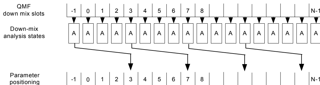
Figure 48 — Stereo down mix analysis procedure
