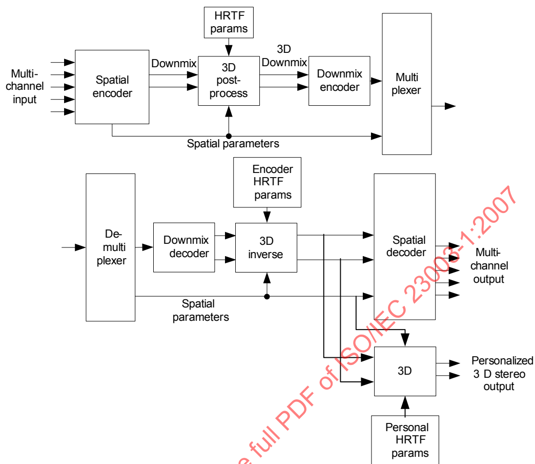
Figure 51 — 3D/binaural downmix as postprocessor of the spatial encoder (upper panel) and inverse 3D/binaural processing in the decoder (lower panel). In addition, Binaural decoding using personalized HRTFs can again be applied to the 3D inverted downmix.
