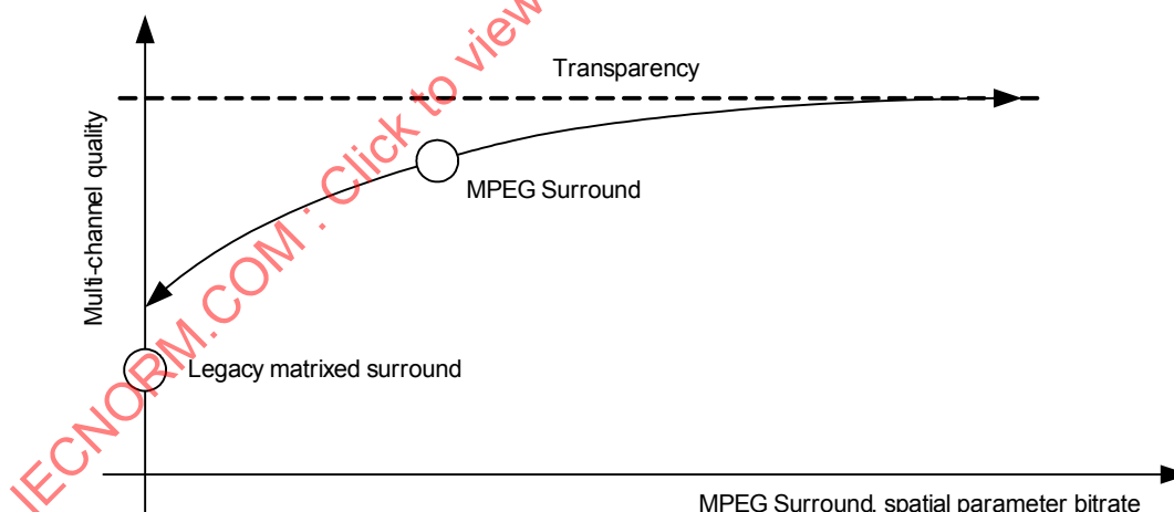
Figure 2 — MPEG Surround bit-rate quality scaling
