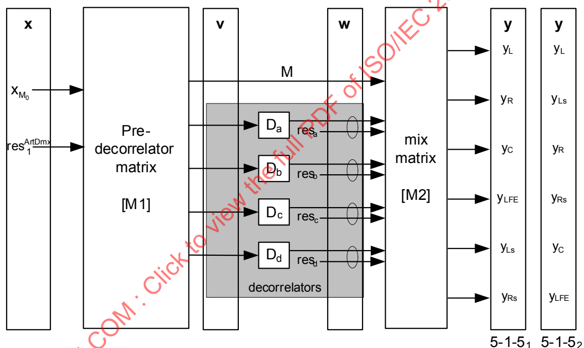
Figure 22 — Matrix view of the spatial audio processing for the 5-1-5 configuration
