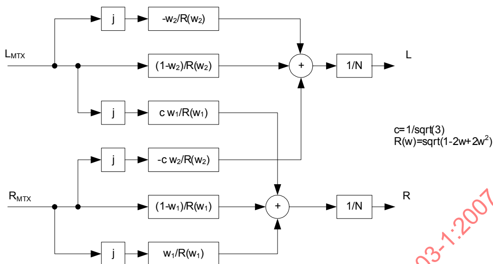
Figure 34 — Matrix compatibility, inversion matrix
