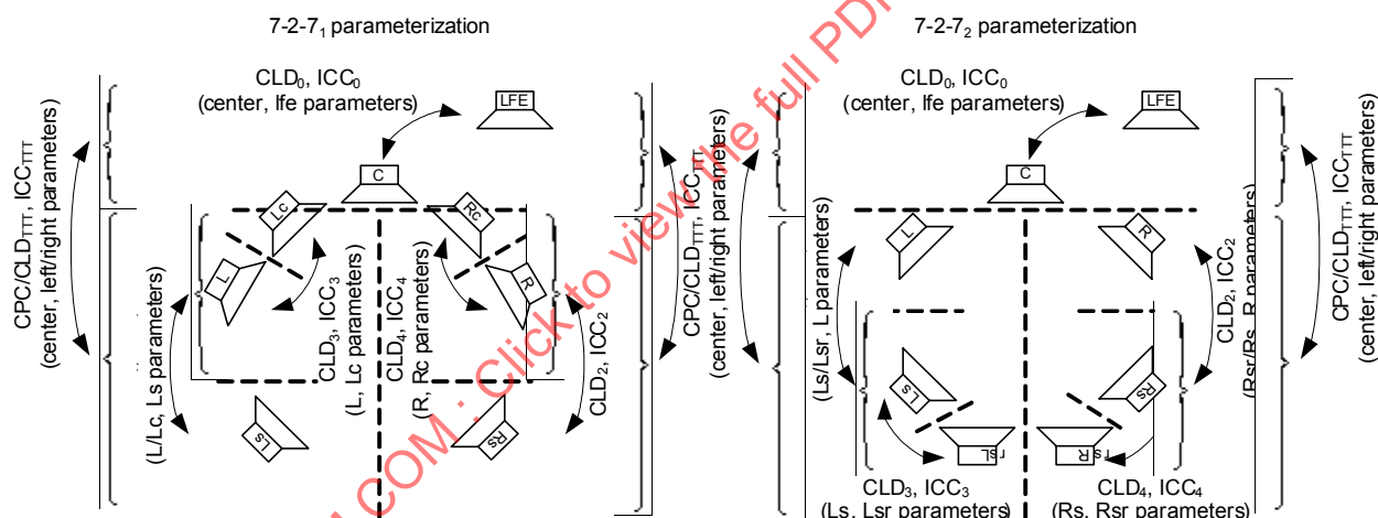
Figure 29 — Parameterization view of the spatial audio processing for the 7-2-7 configurations
