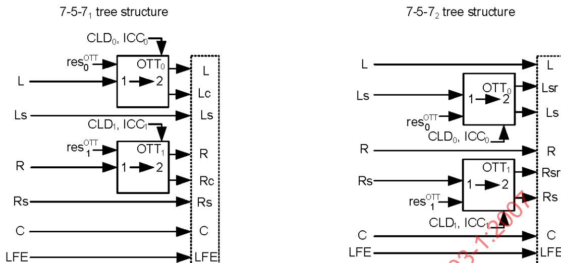
Figure 31 — Tree structure view of the spatial audio processing for the 7-5-7 configurations
