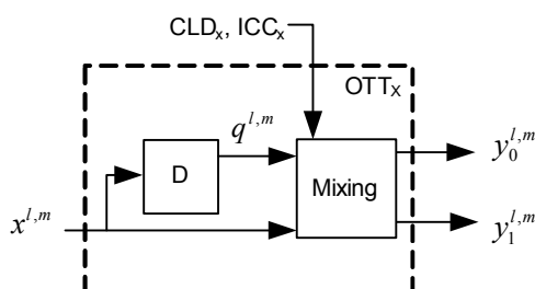
Figure 35 — Equivalent model of a conceptual OTT box
