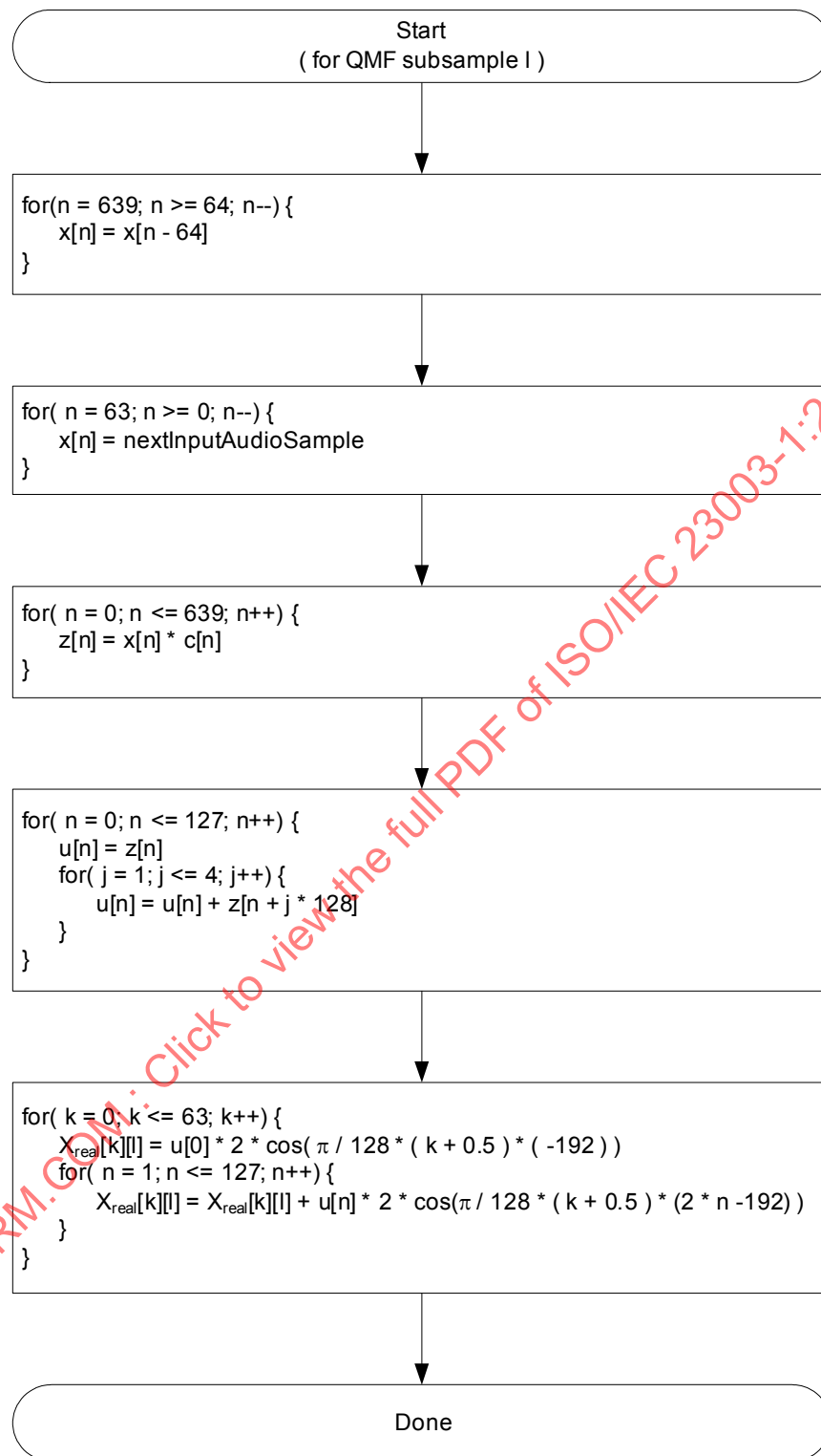
Figure 45 — Flowchart of real-valued analysis QMF bank
