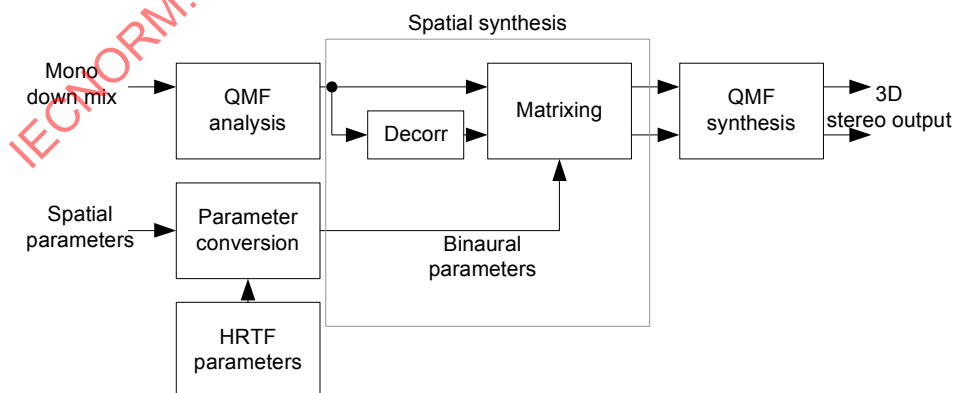
Figure 52 — 3D binaural decoder for '515' spatial configurations
