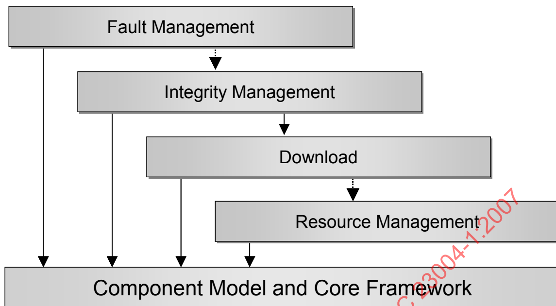
Figure 4 — M3W frameworks
