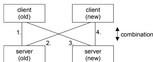
Figure C.4 — Binary compatibility
