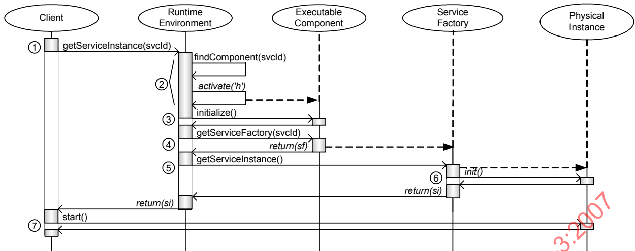
Figure 42 — Service Instance Creation in the Runtime Environment
