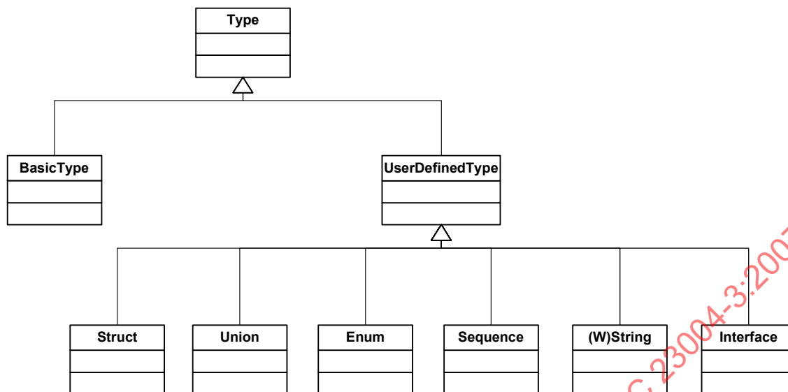
Figure 19 — Types
