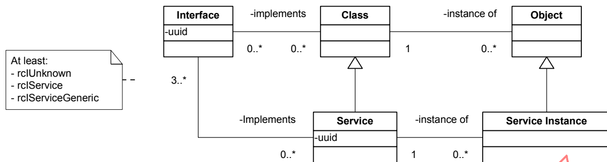
Figure 24 — Service (instance)
