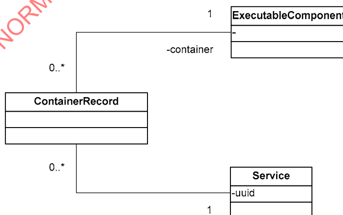
Figure 37 — Service Registration
