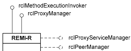
Figure 6 — Interface-Role Model
