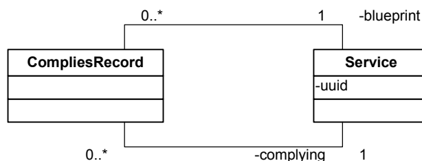
Figure 38 — Complies Registration
