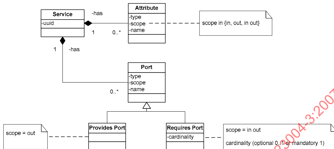
Figure 26 — Ports
