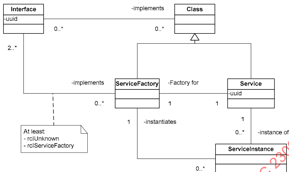
Figure 28 — Service Factory
