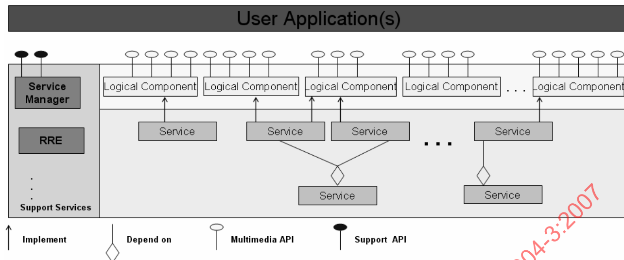
Figure 46 — Logical component and service
