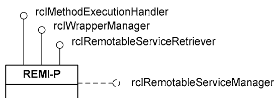
Figure 7 — Interface-Role Model
