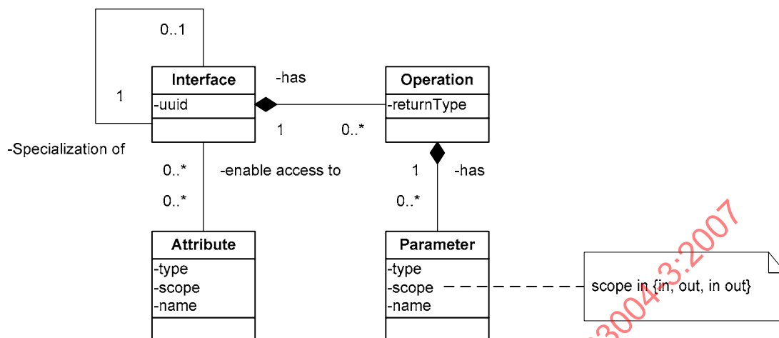
Figure 20 — Interface
