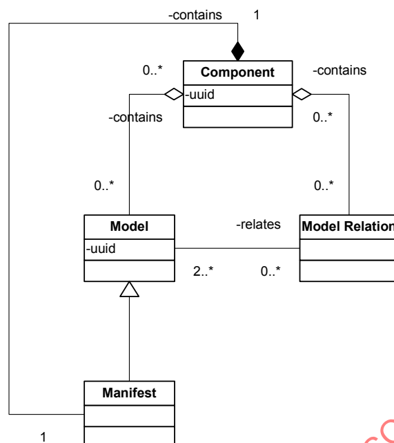
Figure 15 — Component
