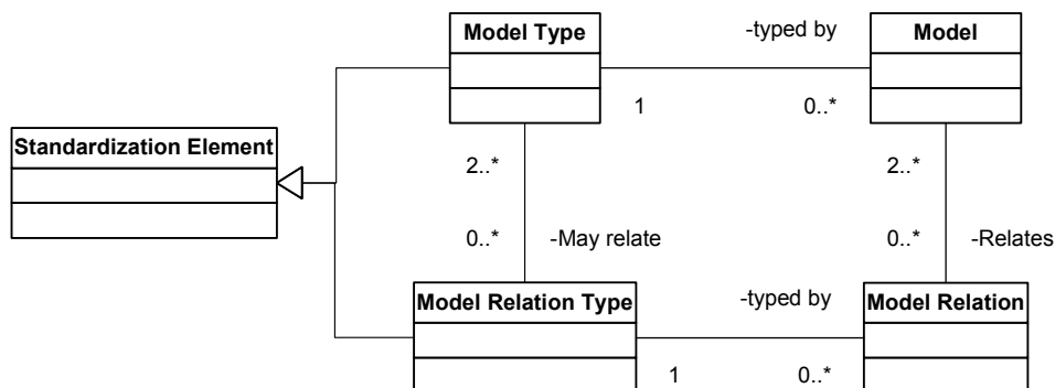
Figure 13 — Model Relation
