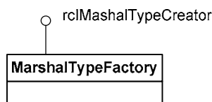
Figure 5 — Interface-Role Model
