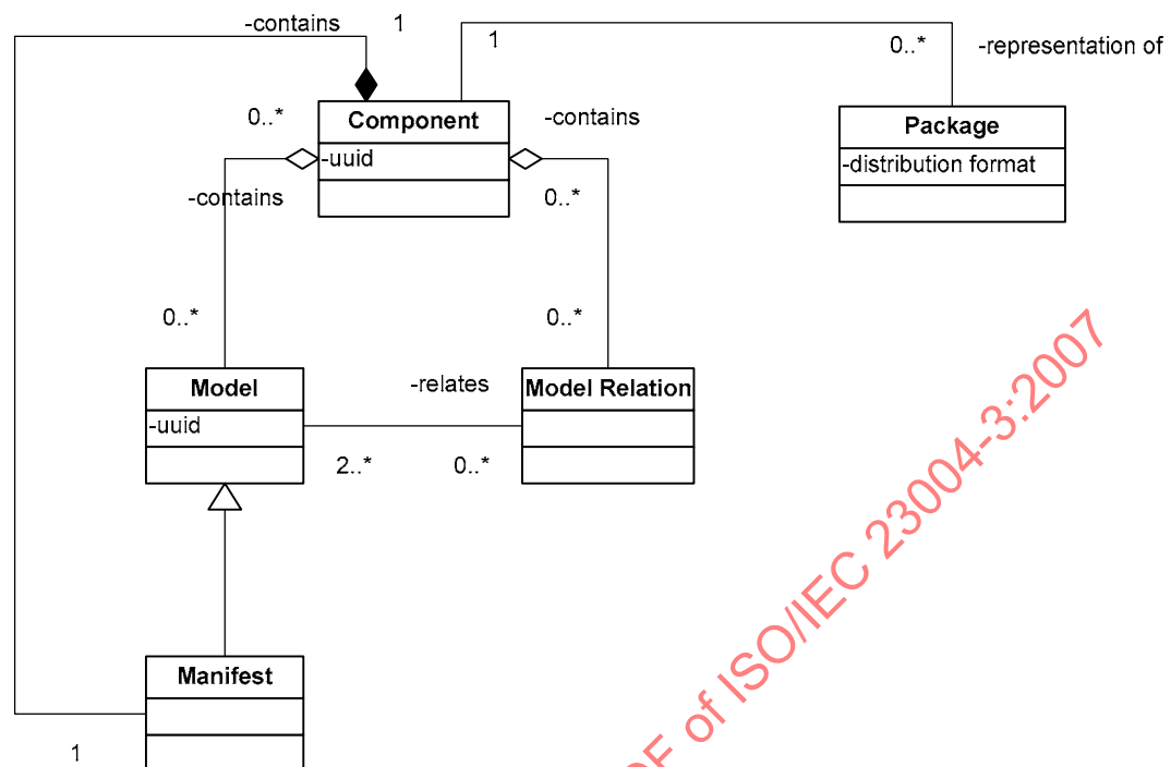
Figure 16 — Package
