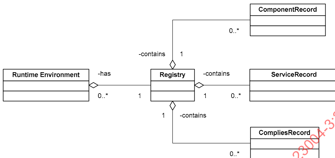
Figure 35 — Registry
