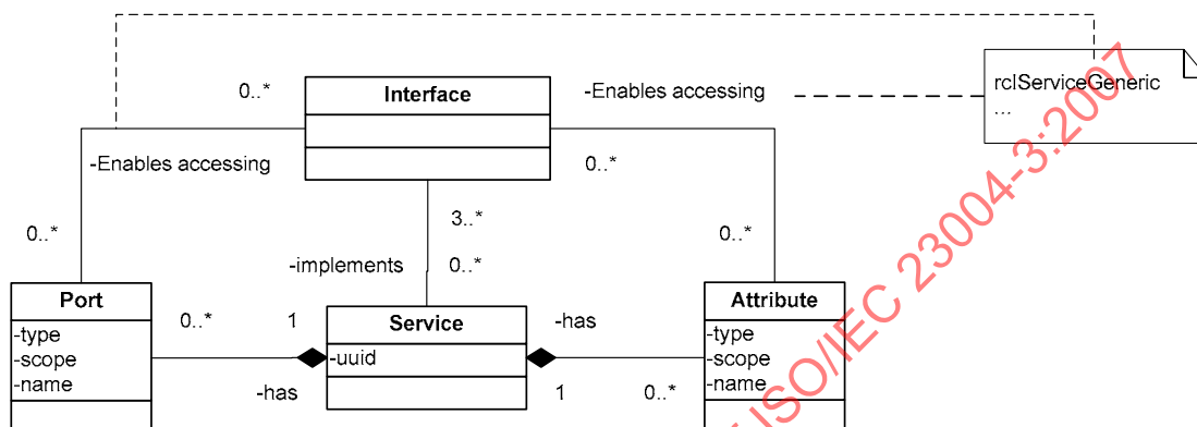
Figure 27 — rcIServiceGeneric interface
