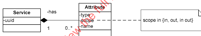
Figure 25 — Attributes
