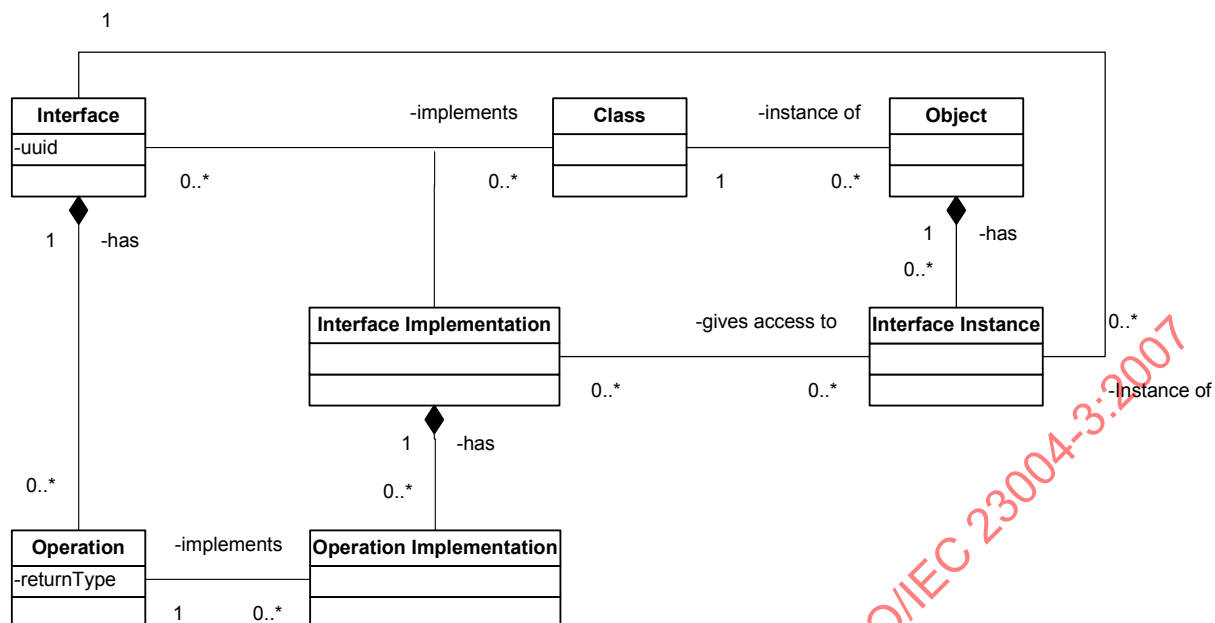
Figure 22 — Interface instance
