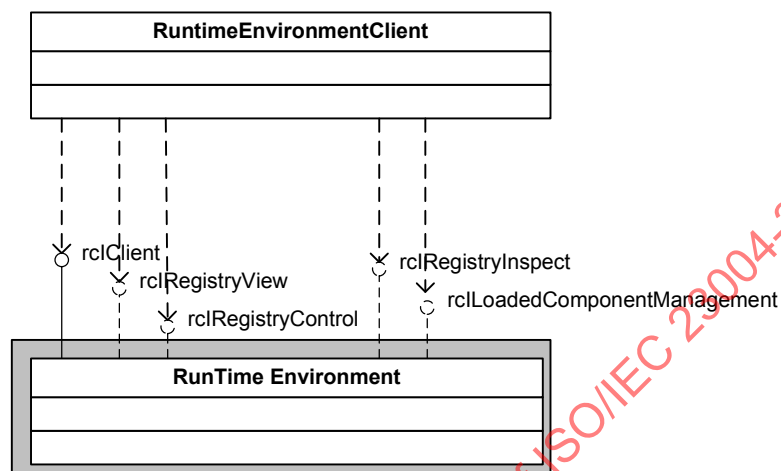
Figure 3 — Interface-Role Model
