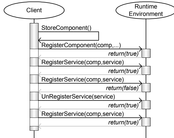
Figure 33 — Registering a Executable Component and its Services
