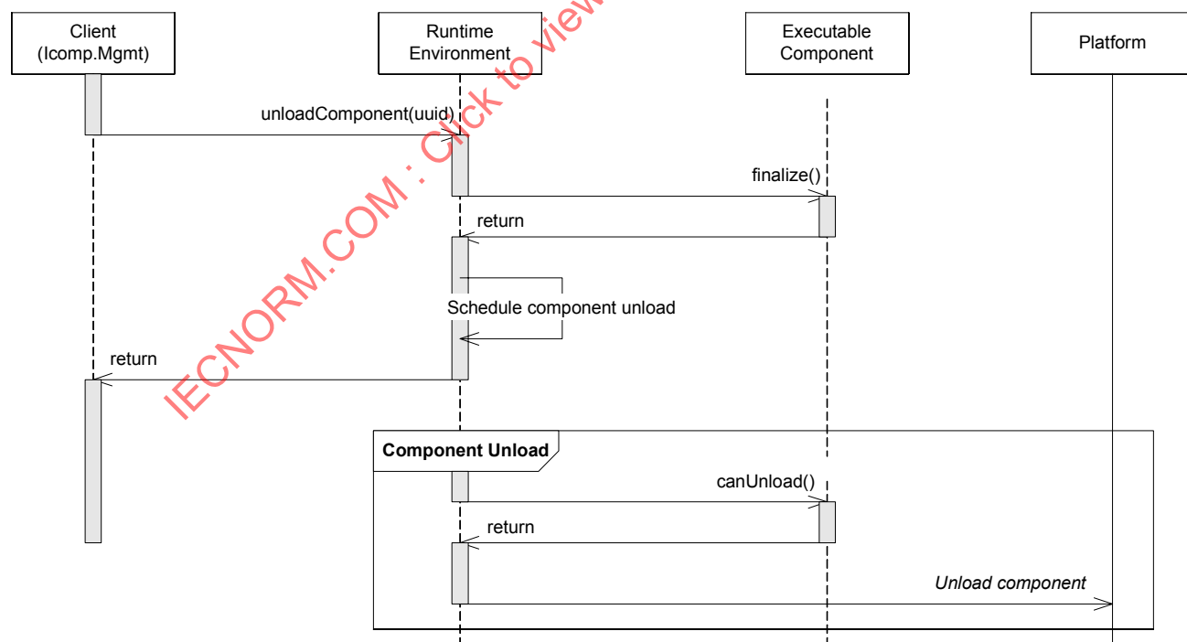
Figure 40 — Explicit client request for Executable Component transition into Unload state
