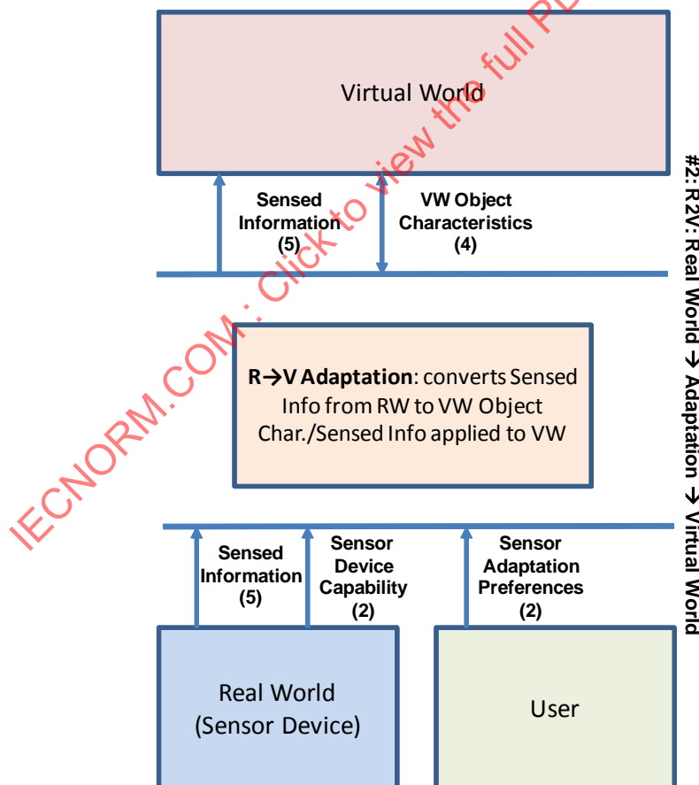
Figure 3 — (Possible) System Architecture for information adaptation from real world to virtual world
