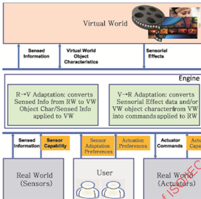
Figure 1 — Scope of the ISO/IEC 23005 series (showing this document in yellow)
