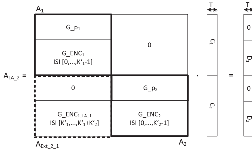
Figure 3 — Encoding process with Layer-Aware RaptorQ constraint matrix A_{LA\_2} for 2 media layers
