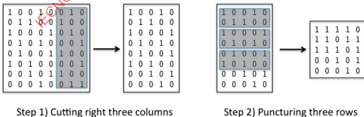
Figure 6 — Puncture operation example to generate punctured matrix ( MK=8 , K'=5 , P'=5 , GC=0 case)
