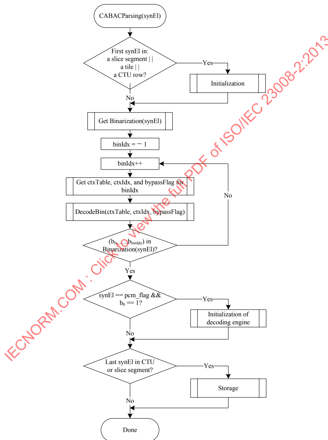
Figure 9-1 – Illustration of CABAC parsing process for a syntax element synEl (informative)
