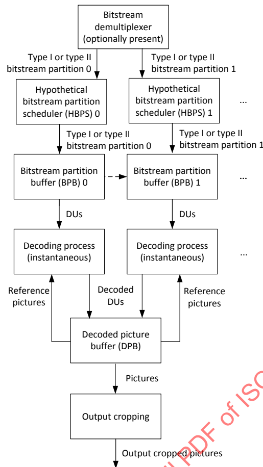
Figure F.1 — Bitstream-partition-specific HRD buffer model
