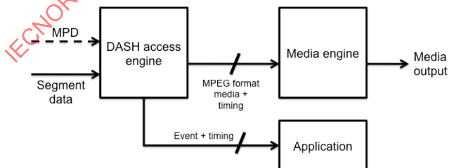
Figure 2 — DASH Client Model
