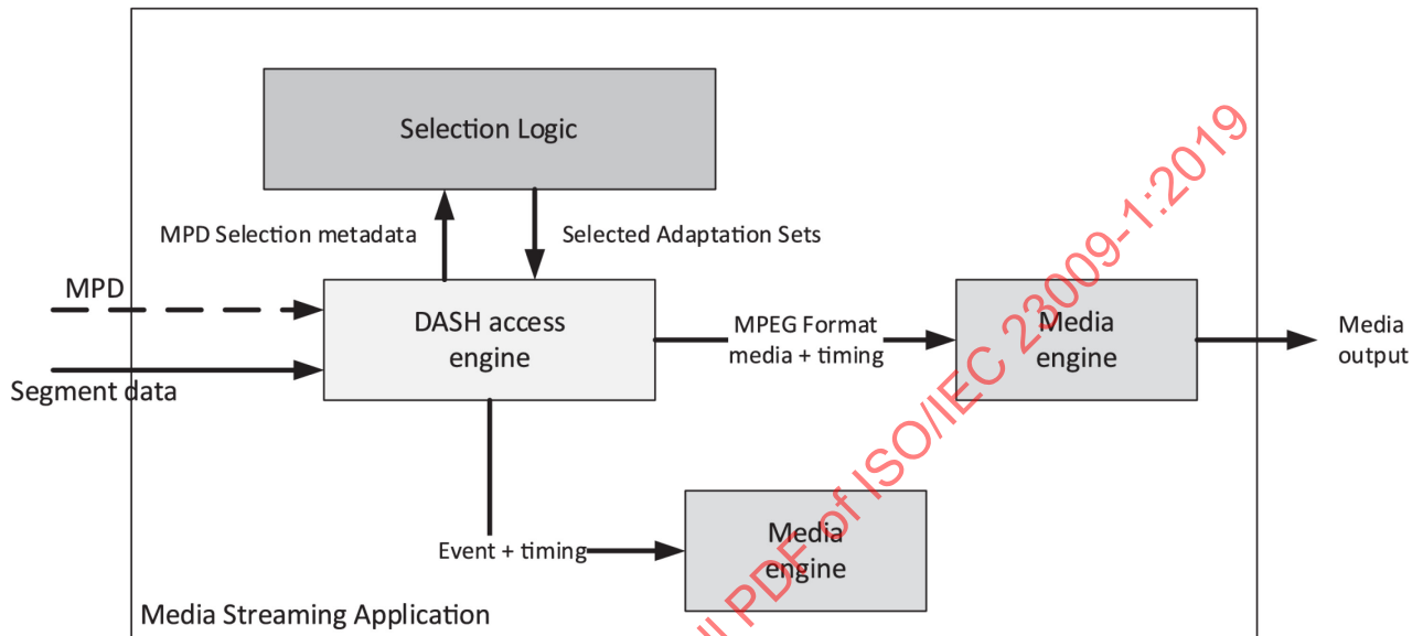
Figure 2 – DASH Client model
