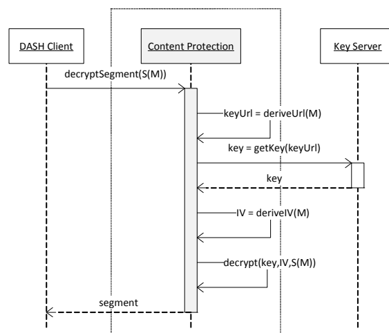
Figure 1 — Baseline Segment Encryption
