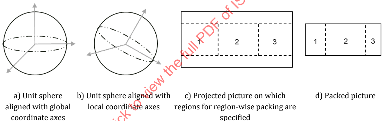
Figure 17 — Example of processing stages to derive a packed picture from a spherical image or vice versa
