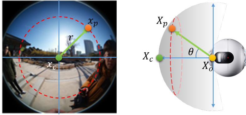
a) Normalized distance ( r ) of a luma sample ( x_p ) on a circular image b) 2D illustration of the definition of the angle ( \theta )
