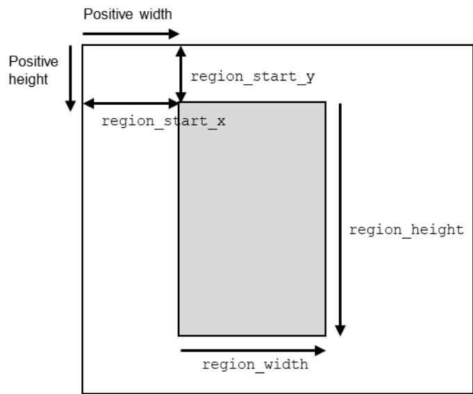
Figure 25 — Rectangular region when region_width and region_height are positive
