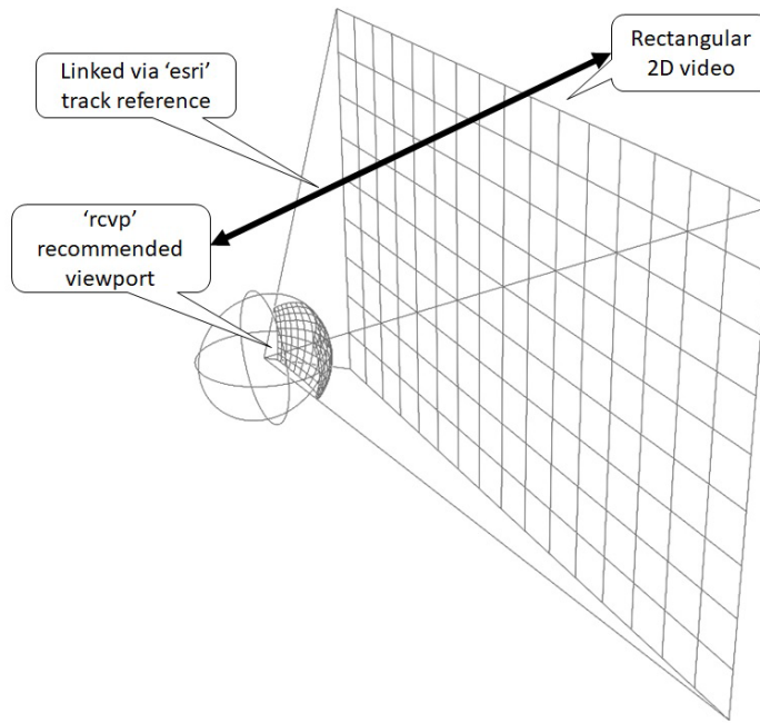
Figure 22 — Illustration of 'esri' track reference
