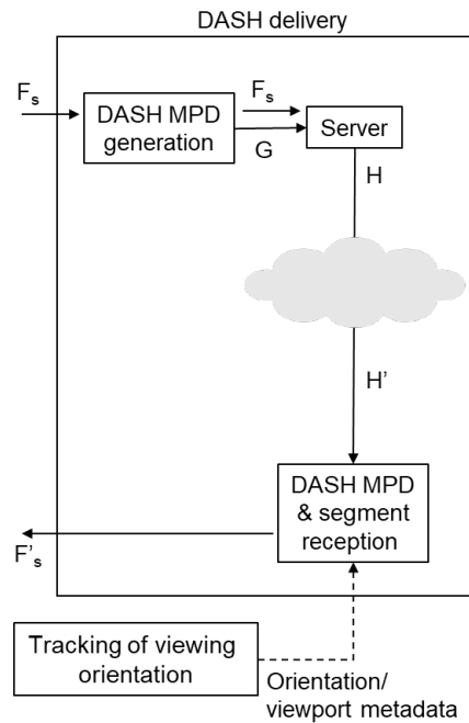
Figure 27 — Illustration of the content flow in the DASH delivery function of OMAF
