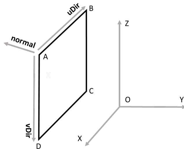
Figure 21 — 3D parallelogram
