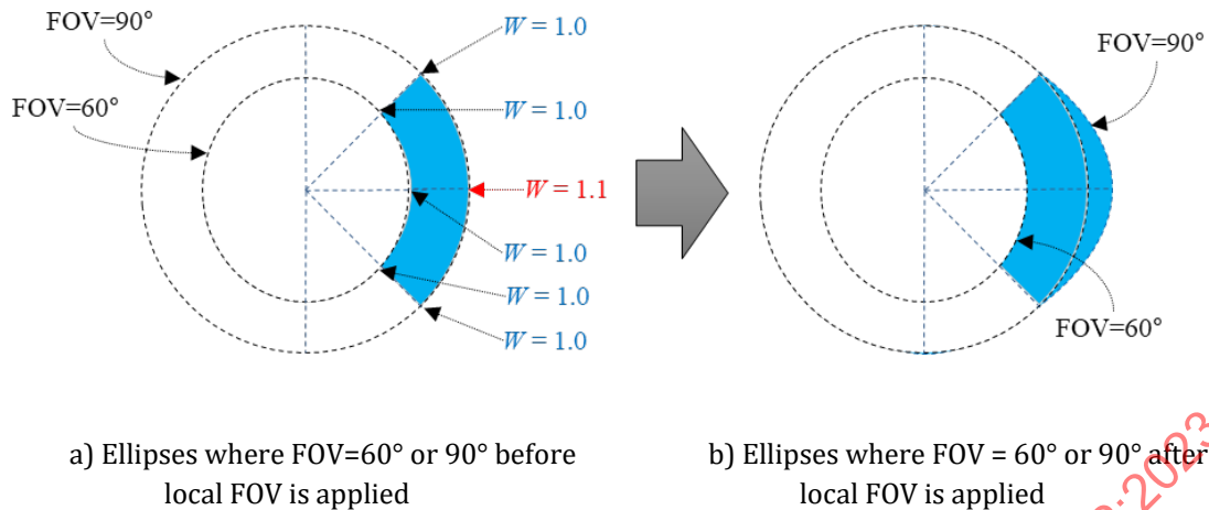
Figure 16 — Example of local FOV with a_s , a_e , and a_d equal to 45°, 135°, and 45°, respectively, and r_s , r_e , and r_d equal to 0.5, 1.0, and 0.5, respectively
