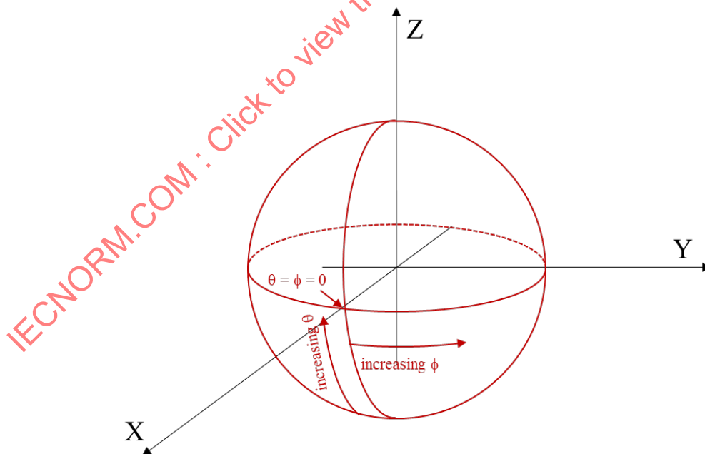
Figure 5 — Coordinate axes and their relation to the sphere coordinates
