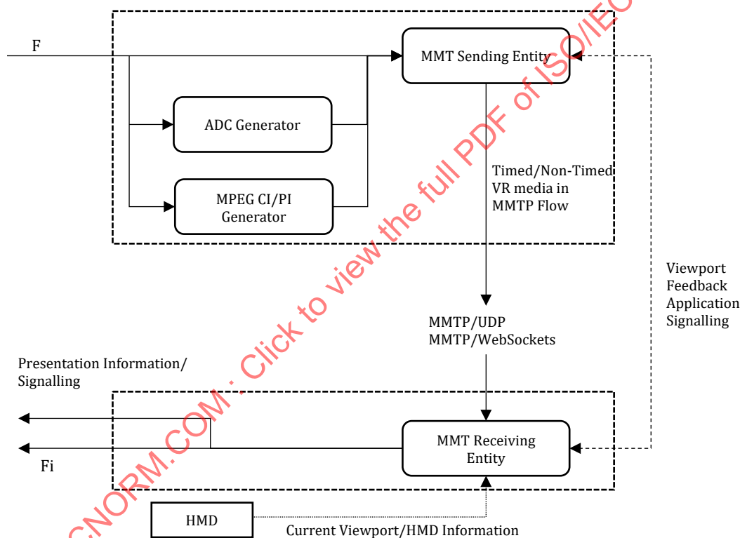
Figure 28 — Reference Architecture for OMAF over MMT
