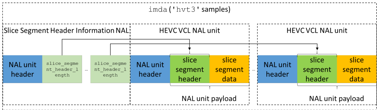
Figure 30 — Slice Segment Header Information NAL-unit-like structure in 'hvt3' tracks
