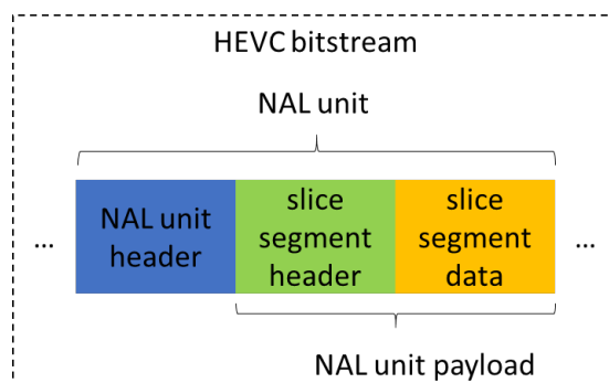
Figure 29 — Video data in HEVC bitstream
