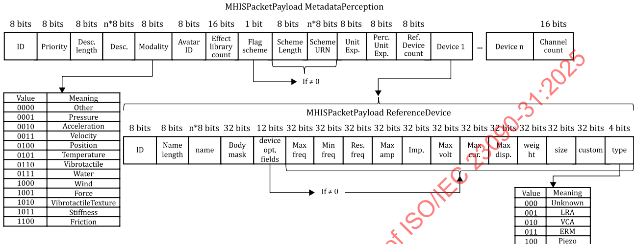
Figure 18 — MIHSPacketPayload structure for packet type PACTYPE_METADATAPERCEPTION
