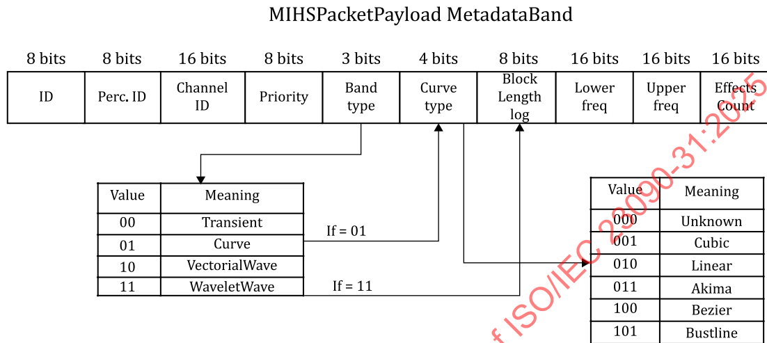
Figure 20 — MIHSPacketPayload structure for packet type PACTYPE_METADATABAND
