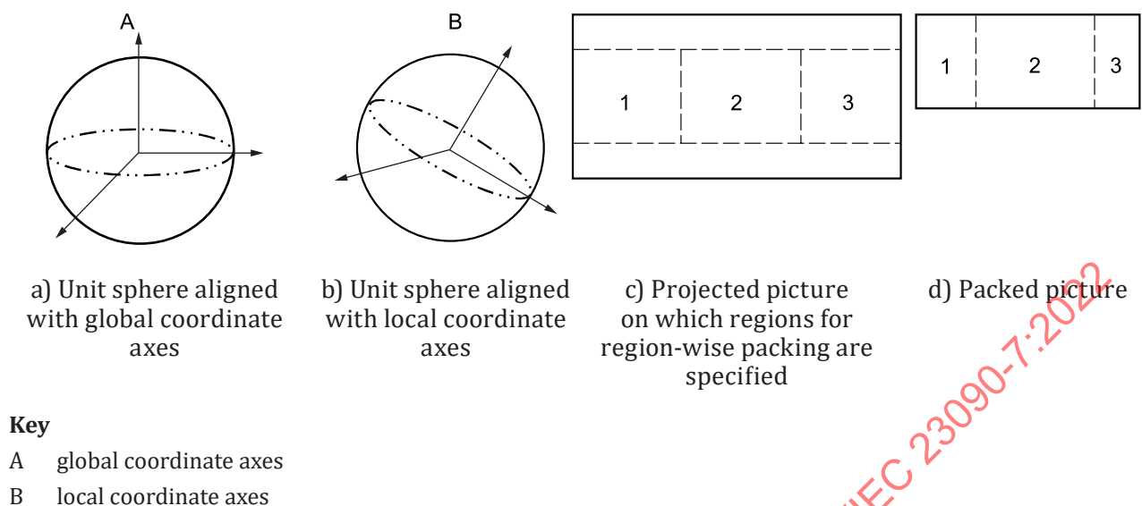
Figure 6.3 — Example of processing stages to derive a packed picture from a spherical image or vice versa
