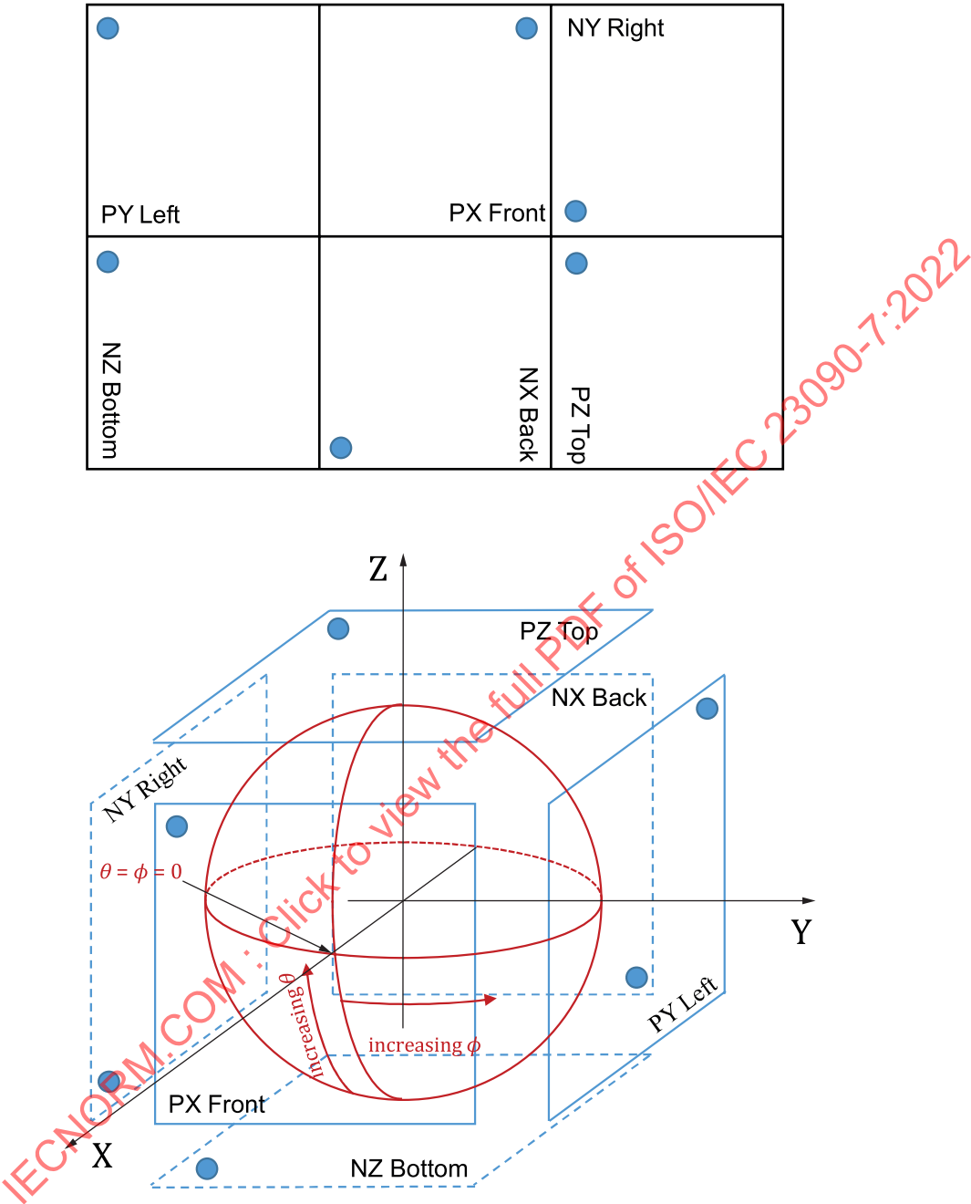
Figure 6.2 — Relation of the cube face arrangement of the projected picture to the sphere coordinates
