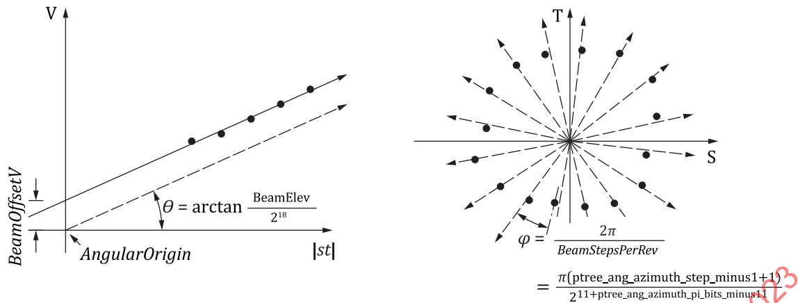
Figure 4 — Origin, elevation angle and azimuth step for a beam
