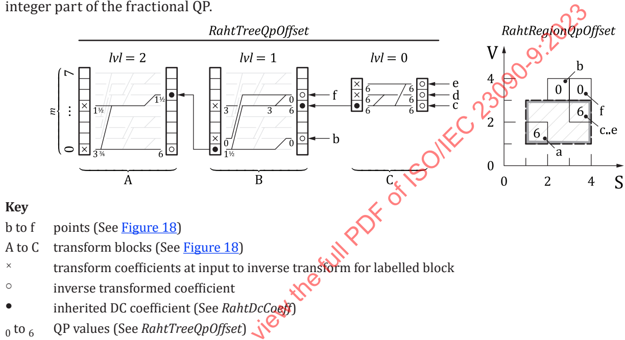
Figure 19 — Example region-dependent QP offset tree
