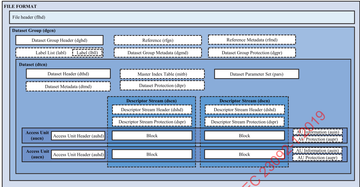
Figure 4 — Data structures hierarchy for storage
