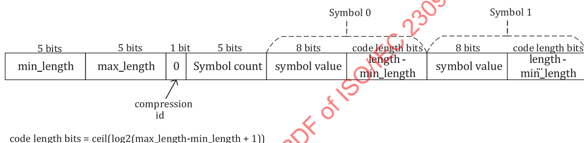
Figure 18 — Prefix coding decoder normal case
