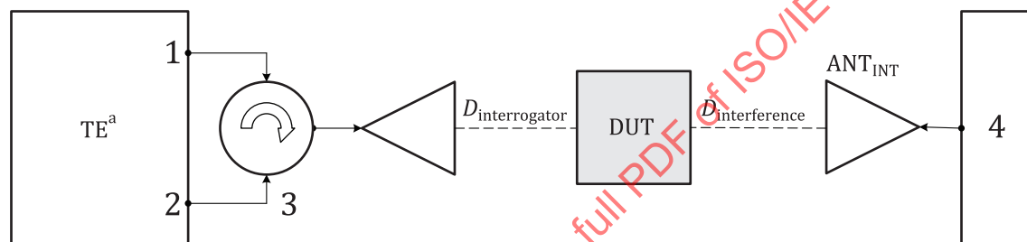
Figure 3 — Bistatic test setup for interference rejection measurement
