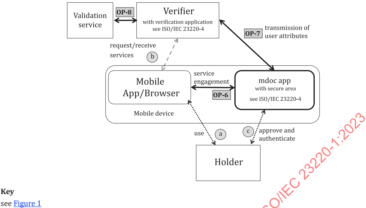
Figure 13 — Remote identification system architecture with local attribute storage with mobile browser
