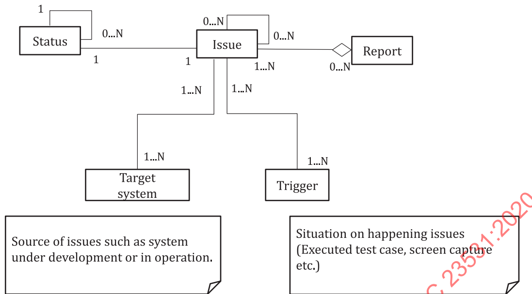
Figure 7 — Class diagram of Common entities
