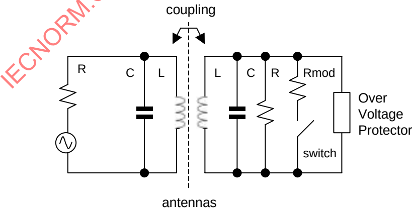
Figure 54 – AIT RMIC interface network
