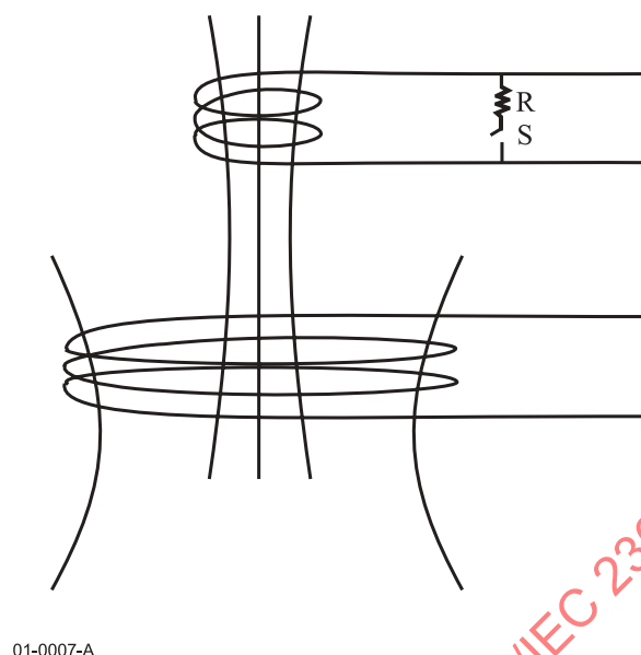
Figure 55 - Illustration of load modulation modulator
