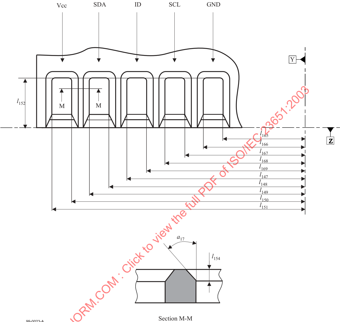
Figure 25 - Case access holes, enlarged partial view, rear side
