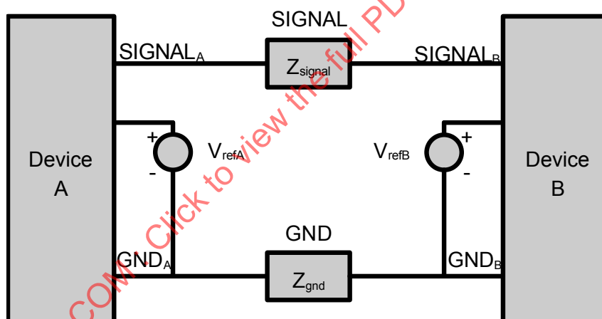
Figure 17 – DC measurements
