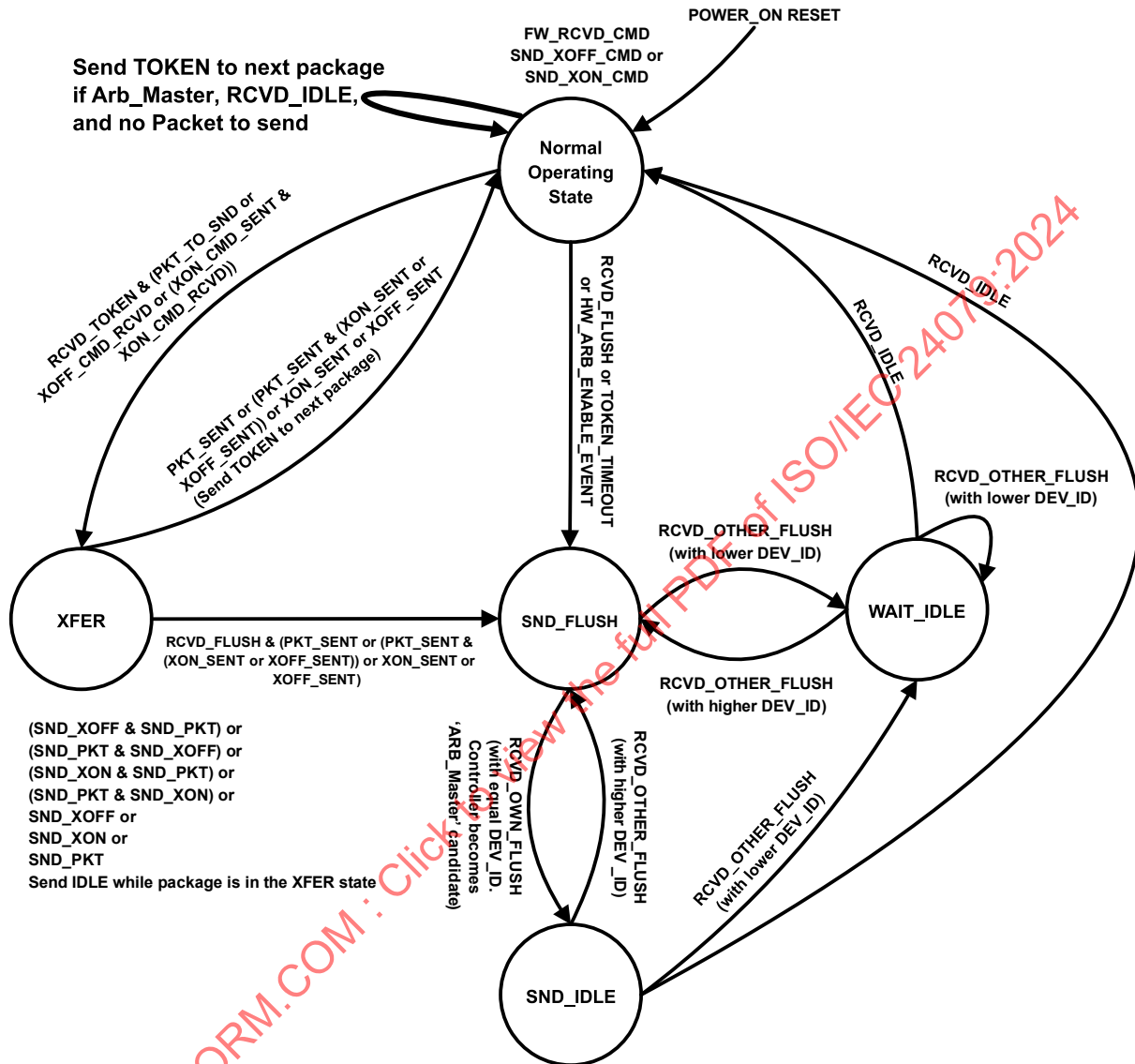
Figure 14 – Hardware arbitration state machine
