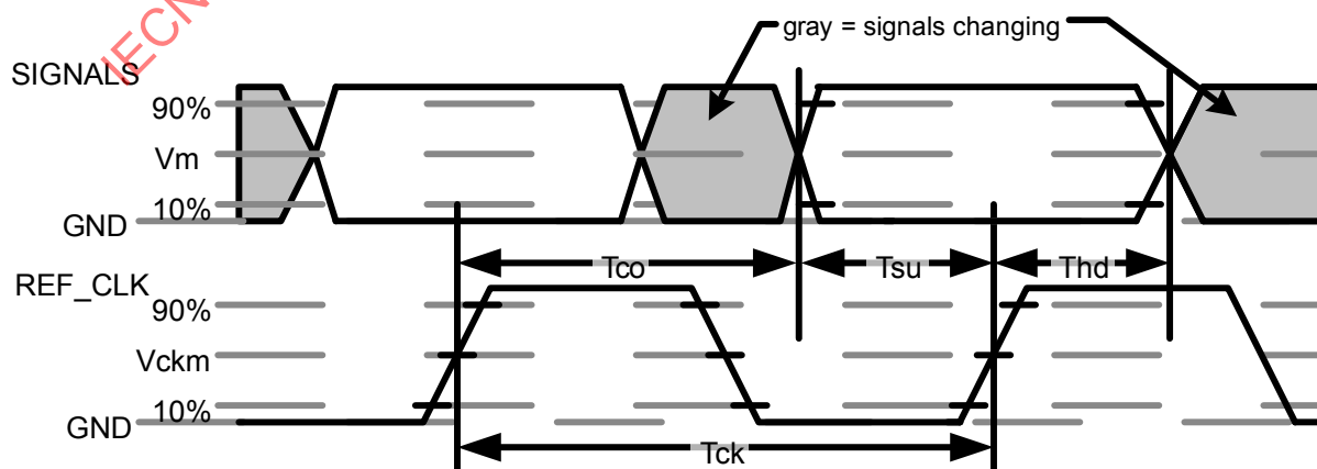
Figure 18 – AC measurements
