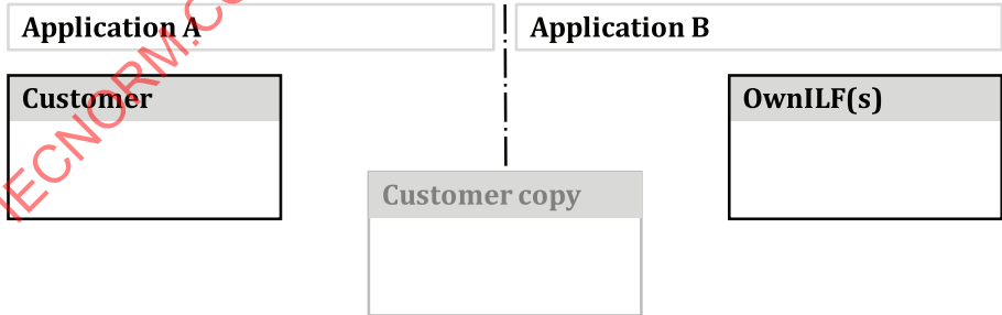
Figure 4.2 — Shared use of data, situation 2
