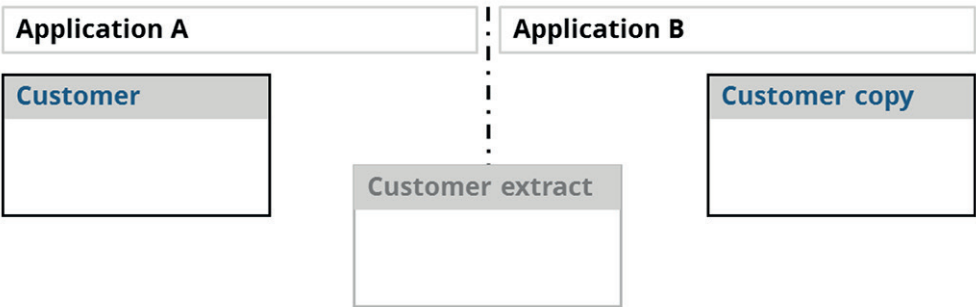
Figure 4.4 — Shared use of data, situation 4
