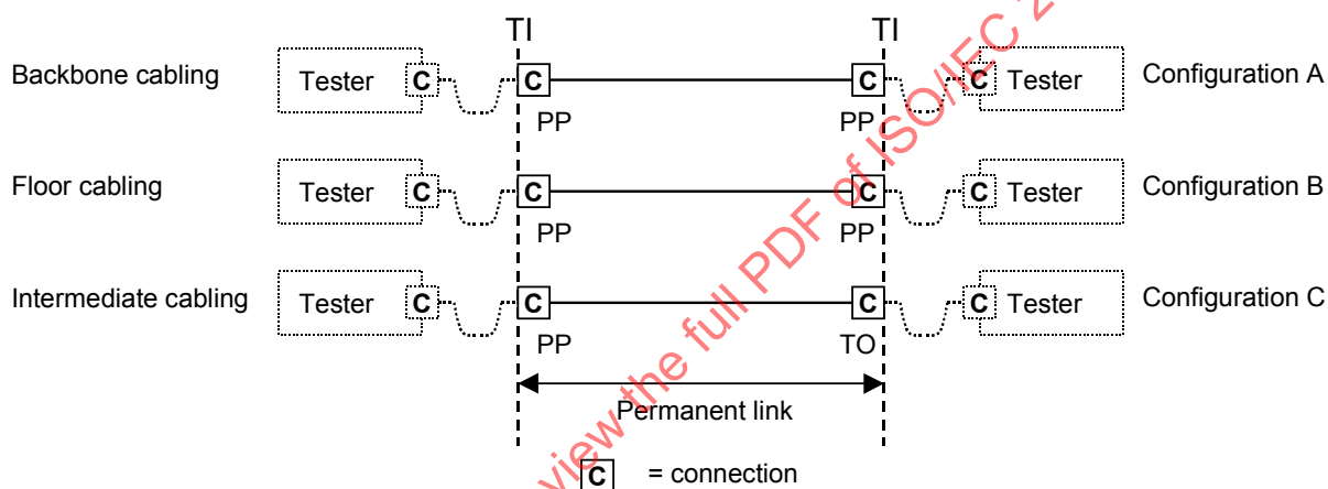
Figure A.1 – Permanent link options
