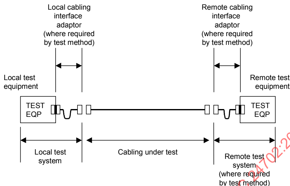
Figure B.2 – The test system and the cabling under test
