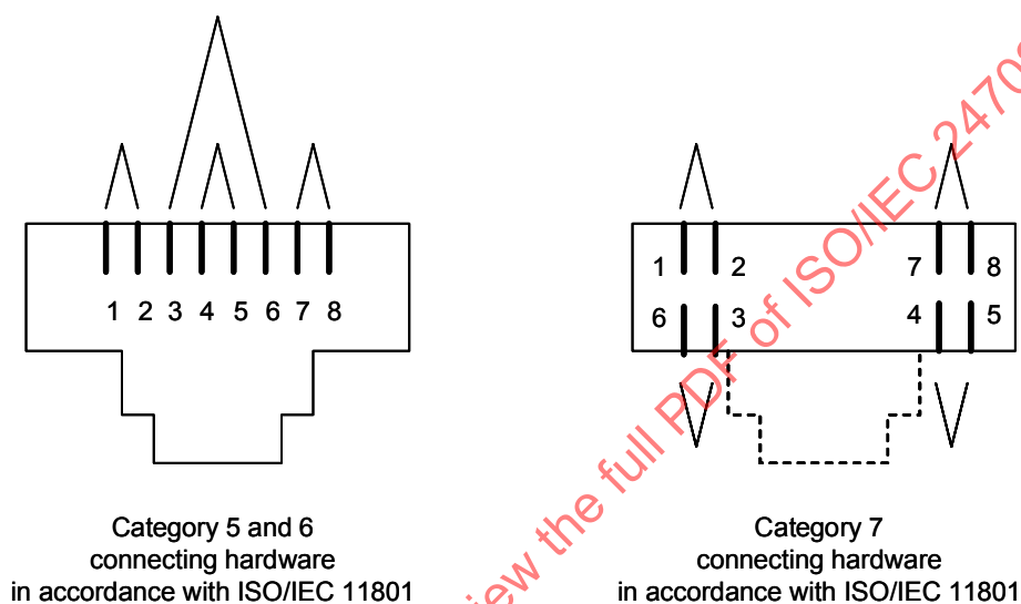
Figure 10 – Eight position jack pin and pair grouping assignments (front view of connector)
