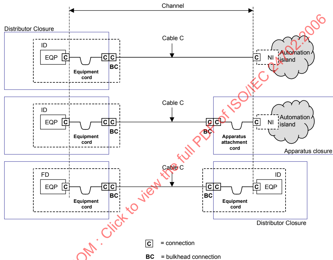
Figure C.3 – Balanced cabling channel configurations with bulkhead connections
