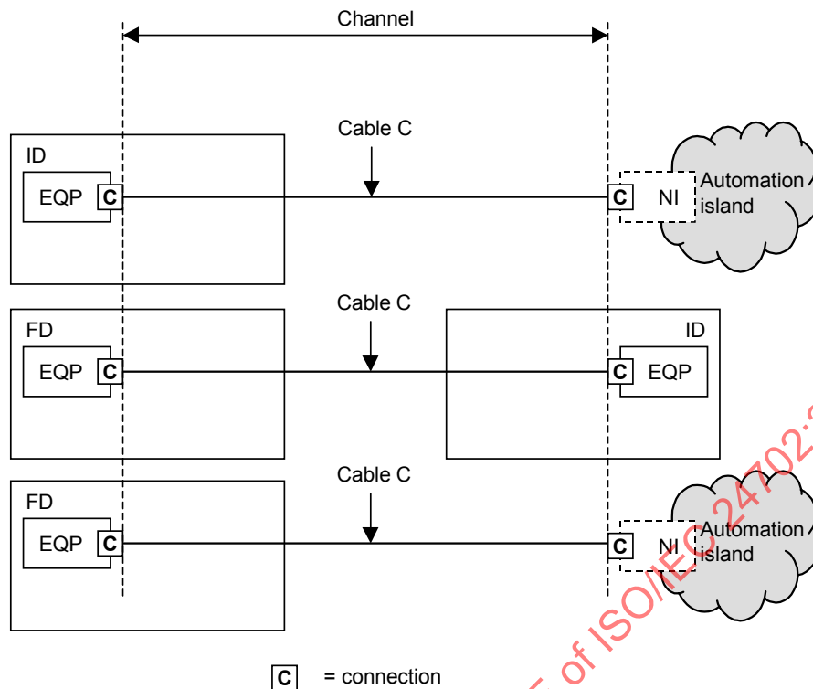
Figure C.1 – Balanced cabling channel configurations with no connections
