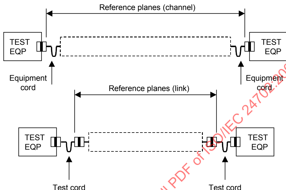
Figure B.1 – Reference planes for link and channels (point-to-point)
