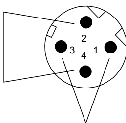
Figure 11 – Four position jack pin and pair grouping assignments (front view of connector)
