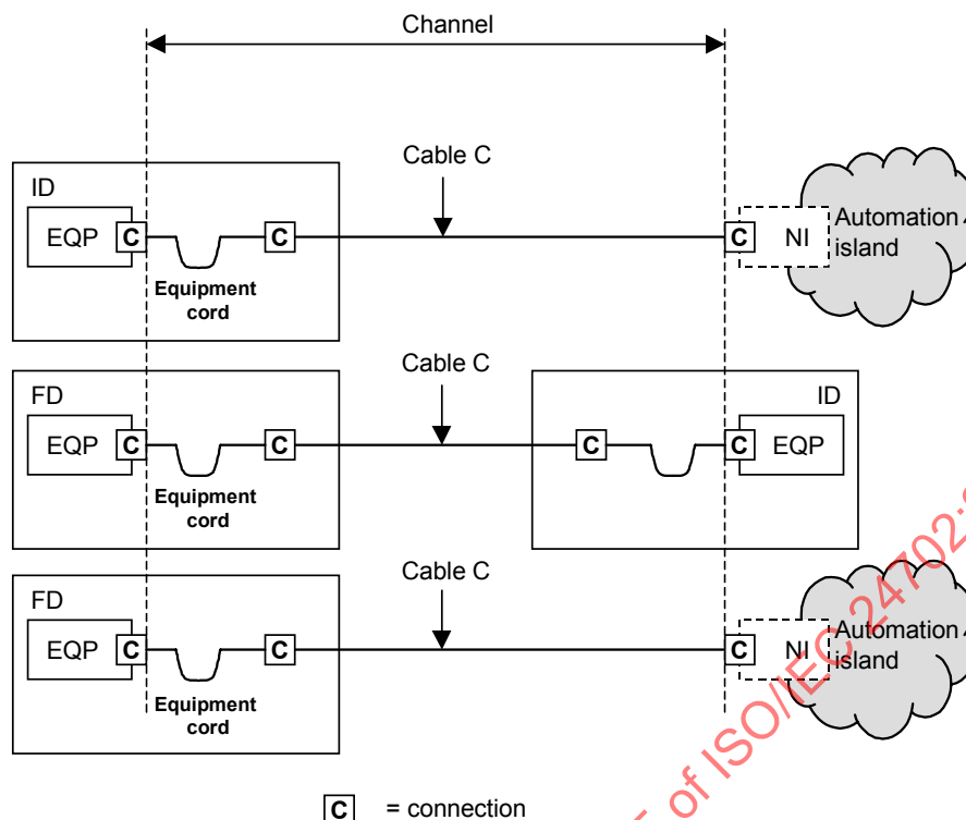
Figure C.2 – Balanced cabling channel configurations of Figure C.1 with interconnection at distributor
