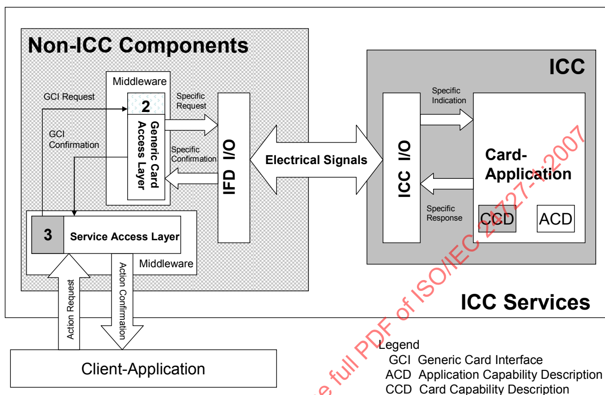
Figure A.2 — Discrete implementation of each interface and layer
