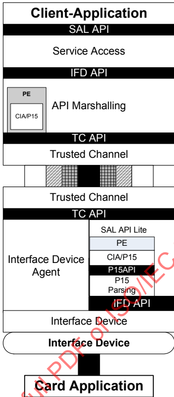
Figure D12 – Proposed Remote-ICC Stack
