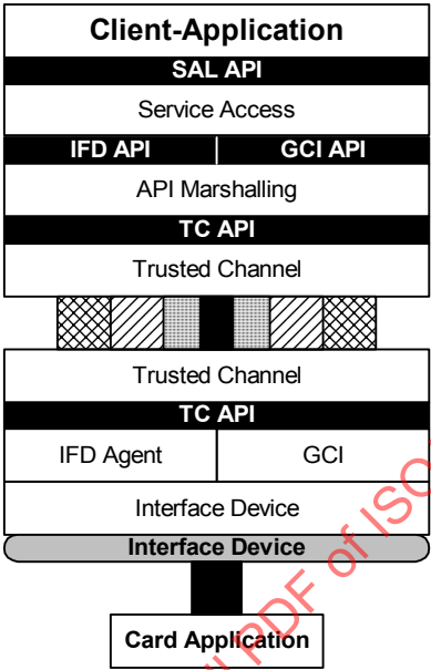
Stack Configuration
