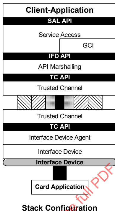
Figure 9 — Remote-ICC-Stack
