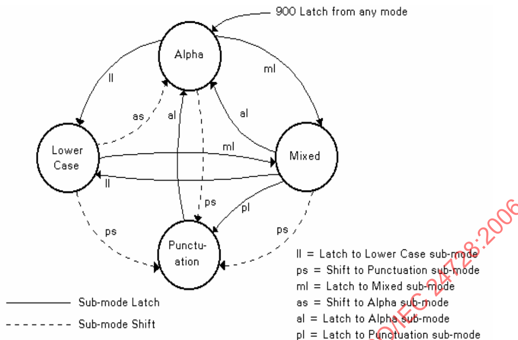
Figure 5 — Text Compaction sub-mode switching
