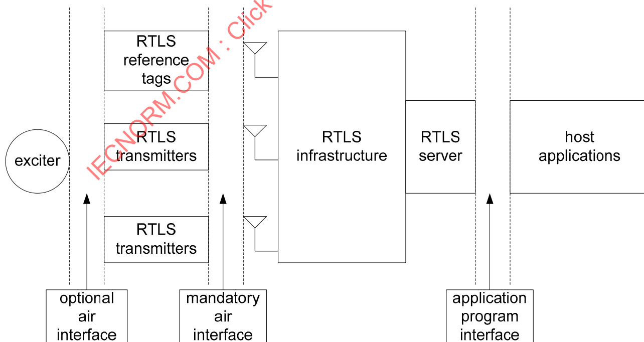
Figure 1 — Elements of RTLS infrastructure
