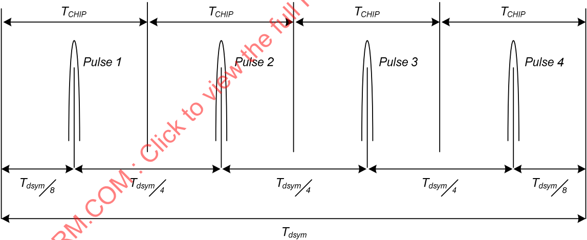
Figure 6 — Extended mode OOK PHY symbol structure
