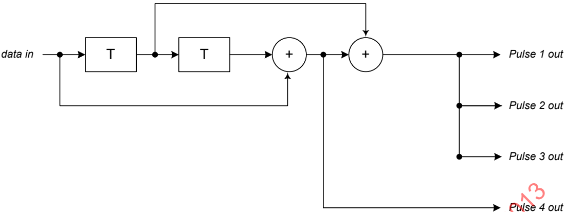
Figure 5 — Extended mode OOK PHY transmitter convolution code
