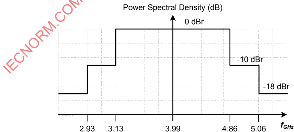
Figure 15 — Transmit spectrum mask for band 4
