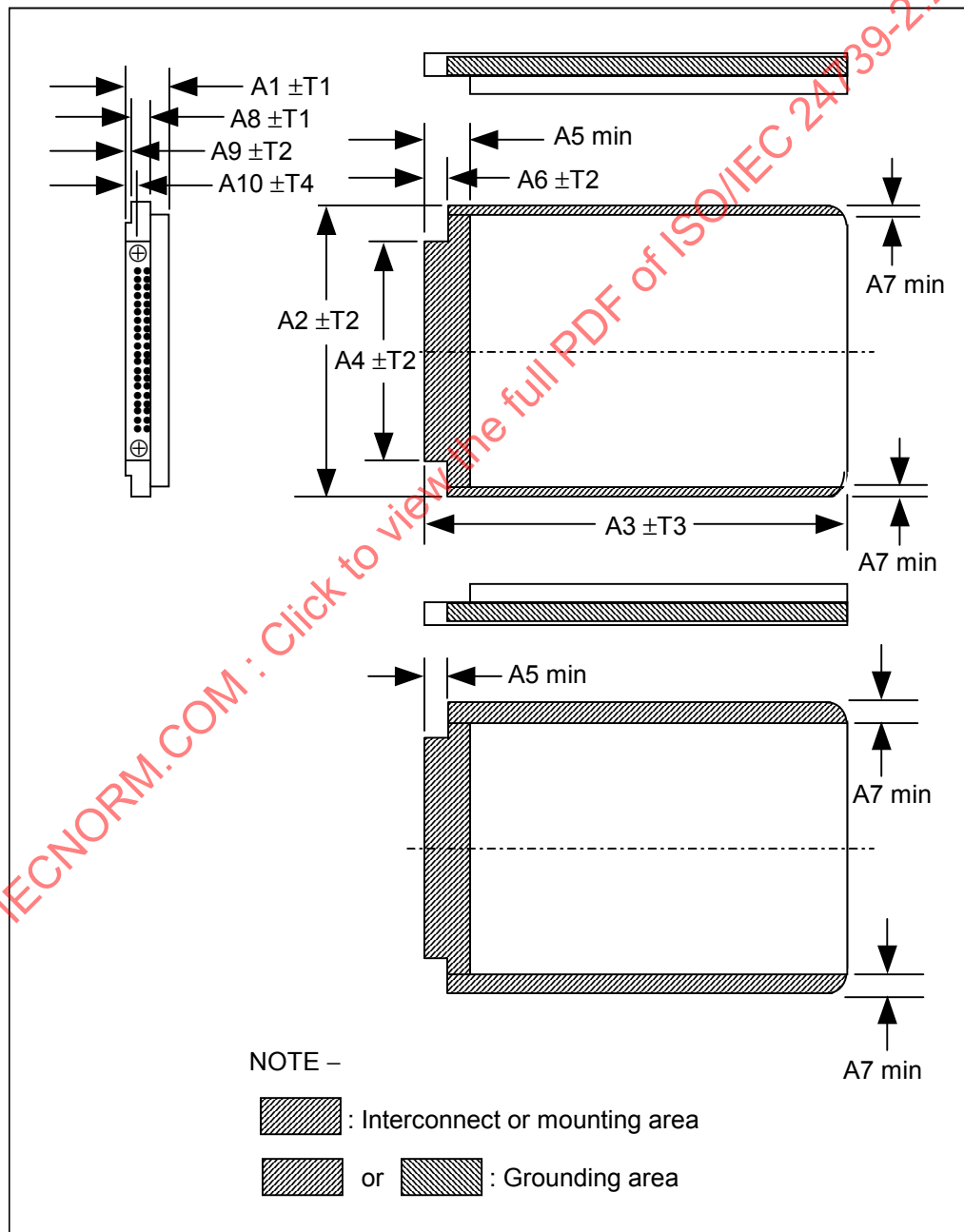
Figure 25 – 48 mm (1.8 in) 3.3 V parallel form factor
