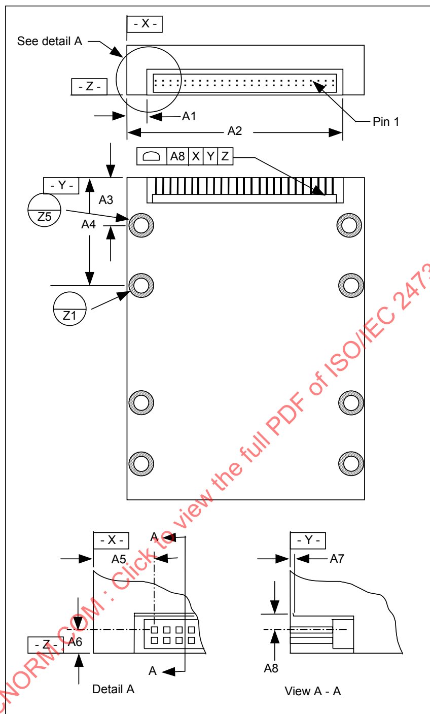
Figure 22 – 65 mm (2.5 in) form factor connector location
