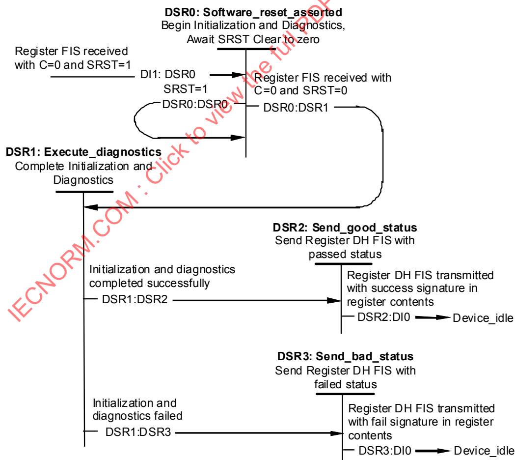
Figure 95 – Software reset protocol (States DSR0-DSR3)
