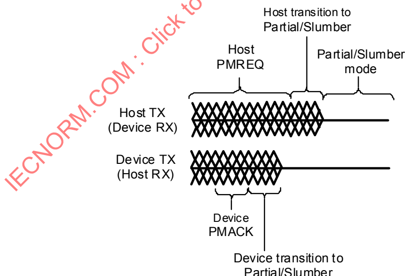
Figure 44 – ON to Partial/Slumber, host initiated
