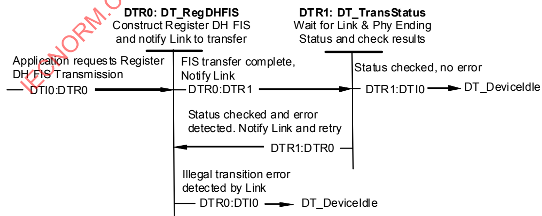
Figure 82 – Device transport send register – Device to host state diagram (DTR0-DTR1)
