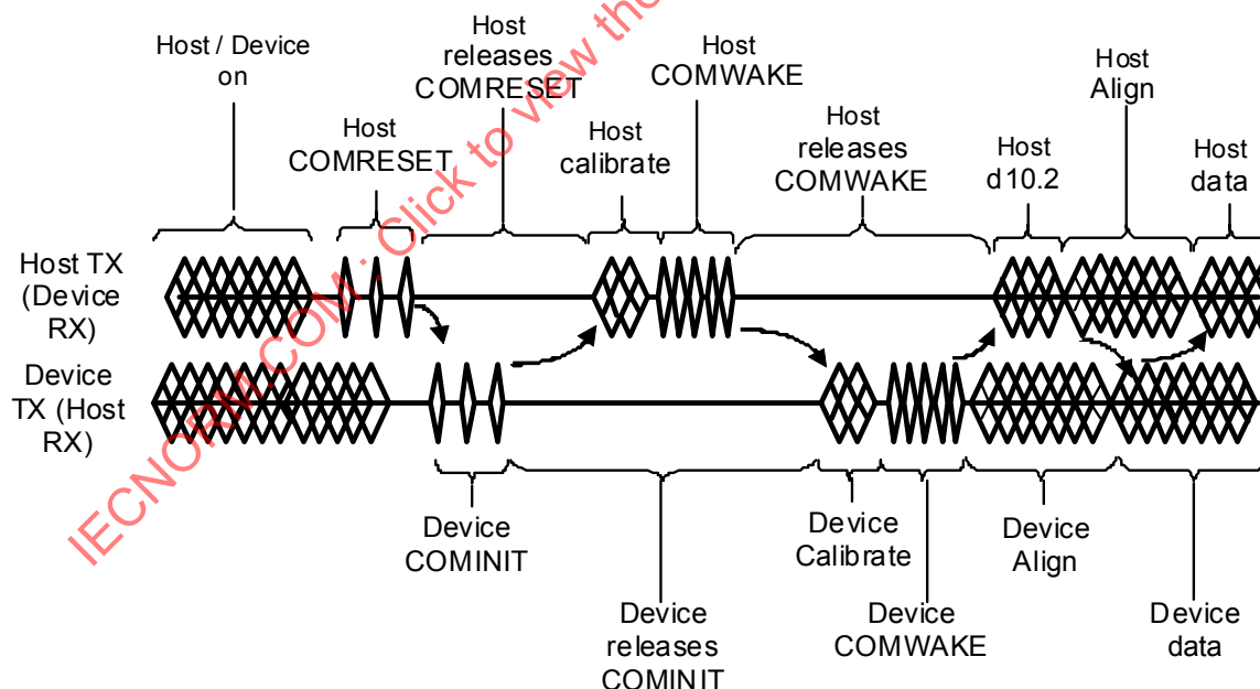
Figure 41 – COMRESET sequence
