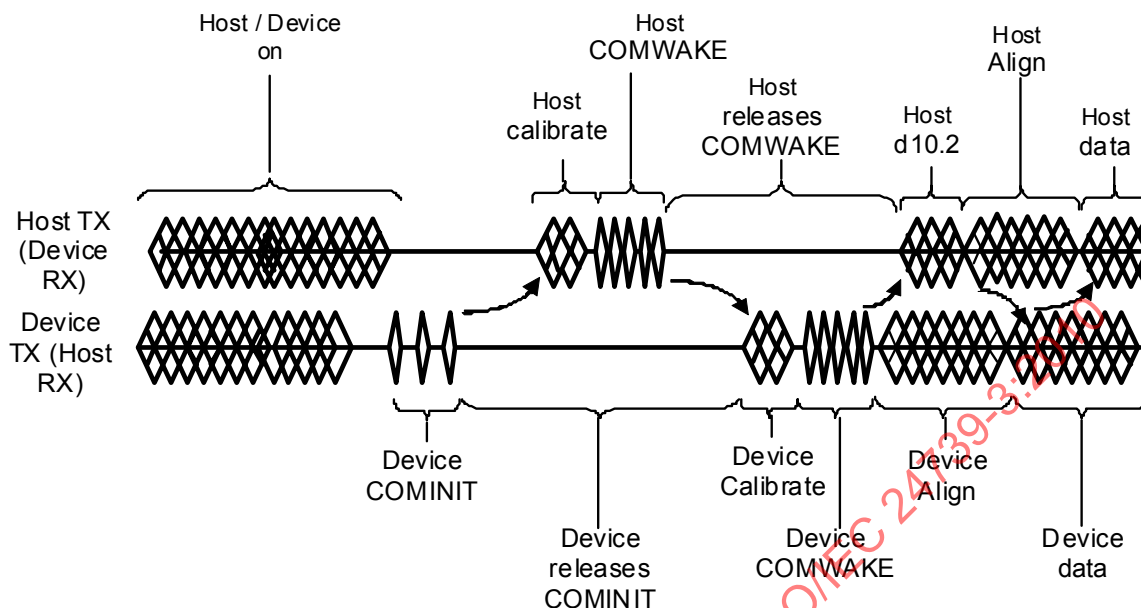
Figure 42 – COMINIT sequence
