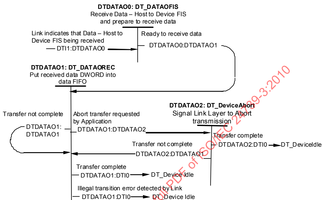
Figure 90 – Device transport decompose data (host to device) FIS state diagram (States DTDATAO0-DTDATAO2)
