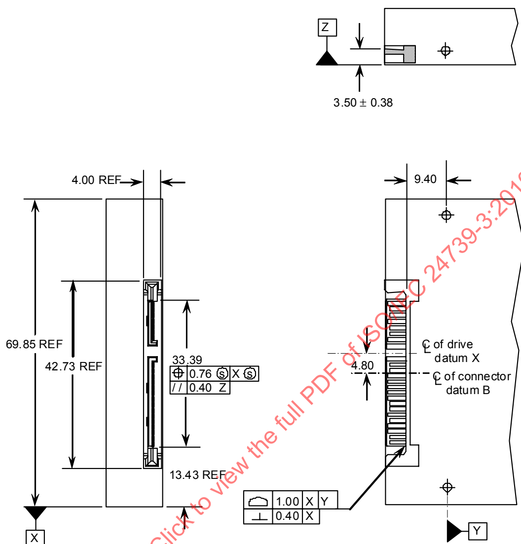
Figure 19 – Device plug connector location on 65 mm (2.5 inch) device
