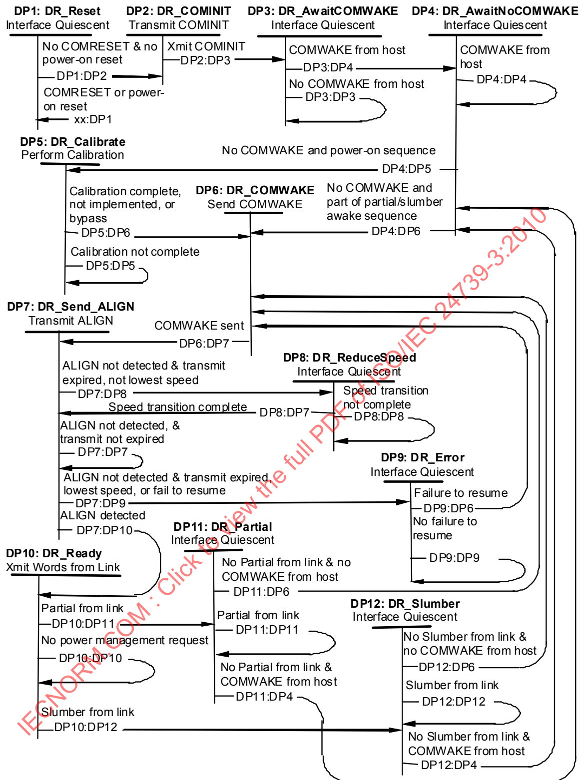
Figure 40 – Device phy initialization state machine (States DP1-DP12)
