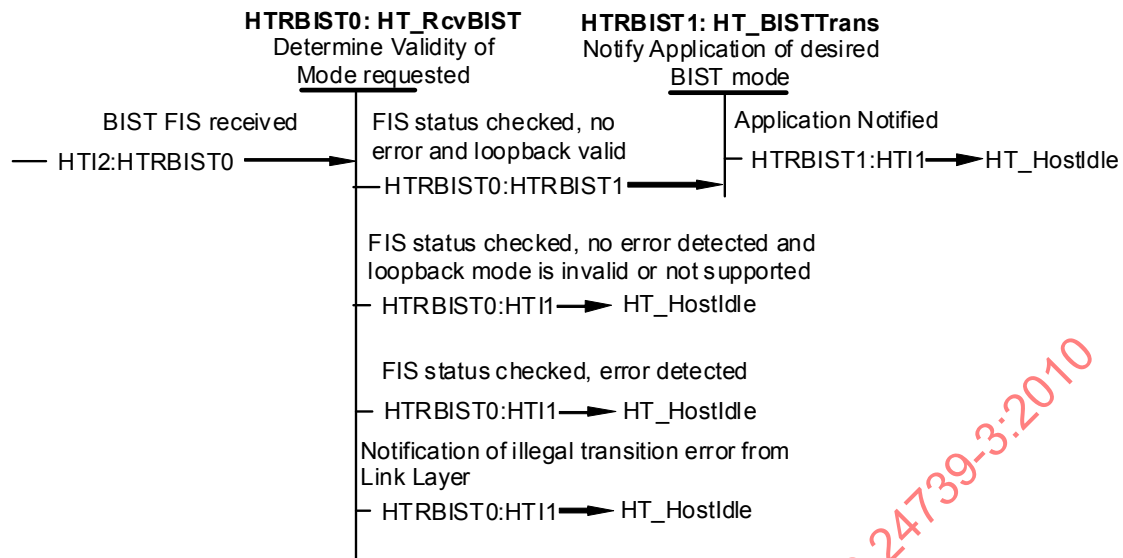
Figure 80 – Host transport decompose BIST activate FIS state diagram (State HTRBIST0-HTRBIST1)
