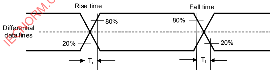
Figure 30 – Signal rise and fall times
