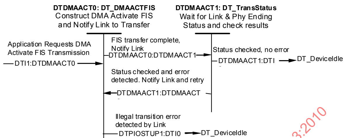
Figure 85 – Device transport transmit DMA activate FIS state diagram (States DTDMAACT0-DTDMAACT1)
