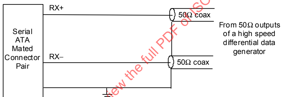
Figure 32 – Receive test fixture
