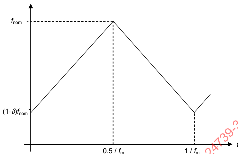
Figure 36 – Triangular frequency modulation profile
