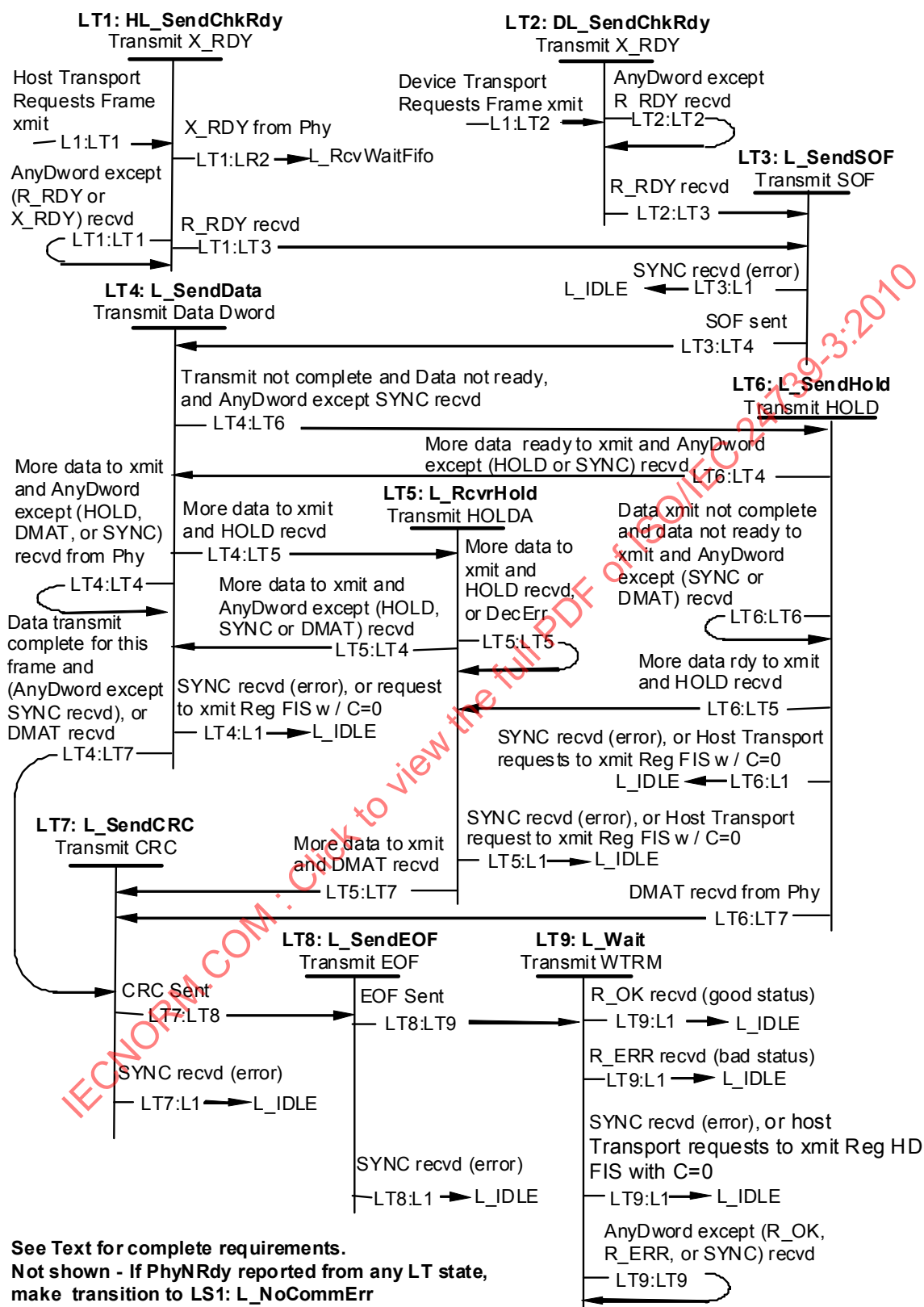
Figure 59 – Link transmit state diagram (States LT1-LT9)
