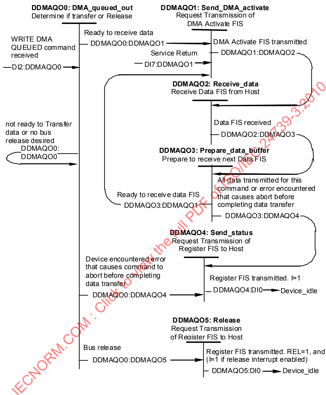
Figure 105 – WRITE DMA QUEUED command protocol (DDMAQ00-DDMAQ05)
