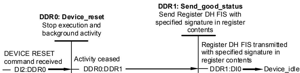
Figure 97 – DEVICE RESET command protocol (States DDR0-DDR1)
