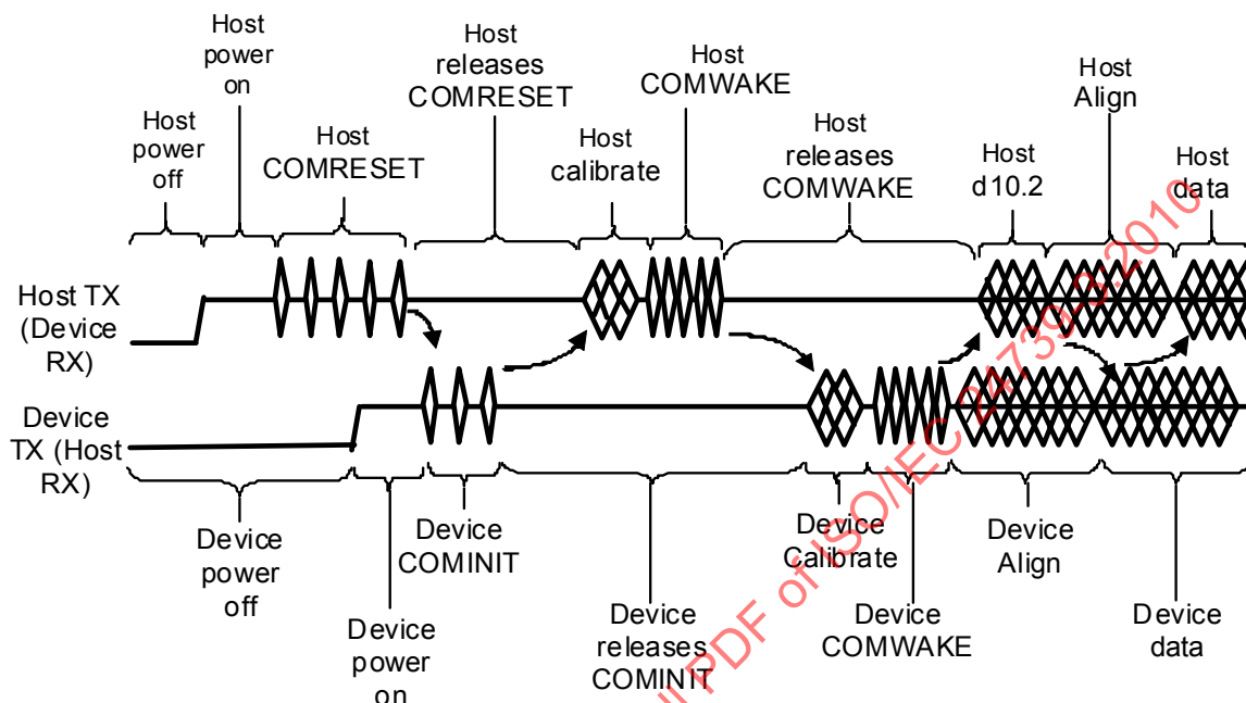
Figure 43 – Power-on sequence
