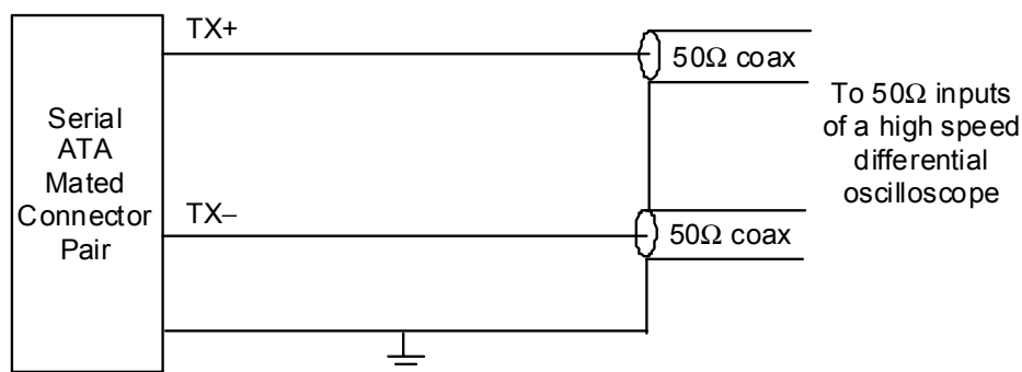
Figure 31 – Transmit test fixture
