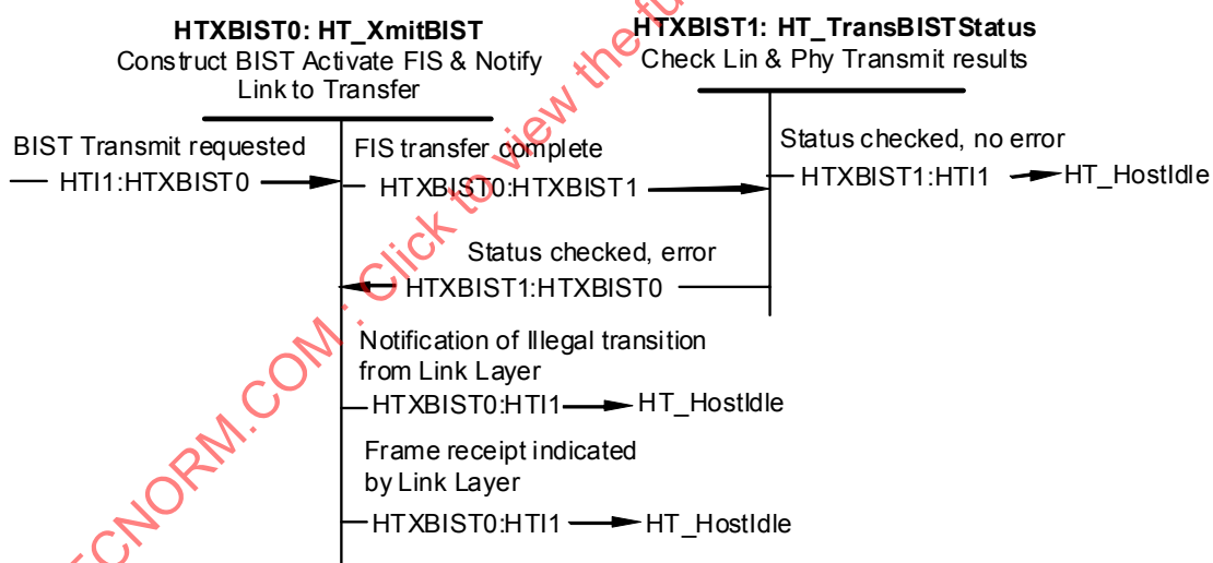
Figure 74 – Host transport transmit BIST activate FIS (States HTXBIST0-HTXBIST1)
