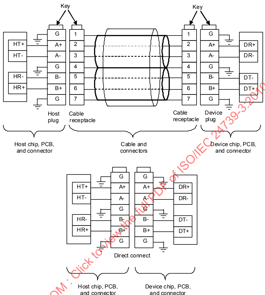
Figure 22 – Signals and grounds assigned in direct connect and cabled
