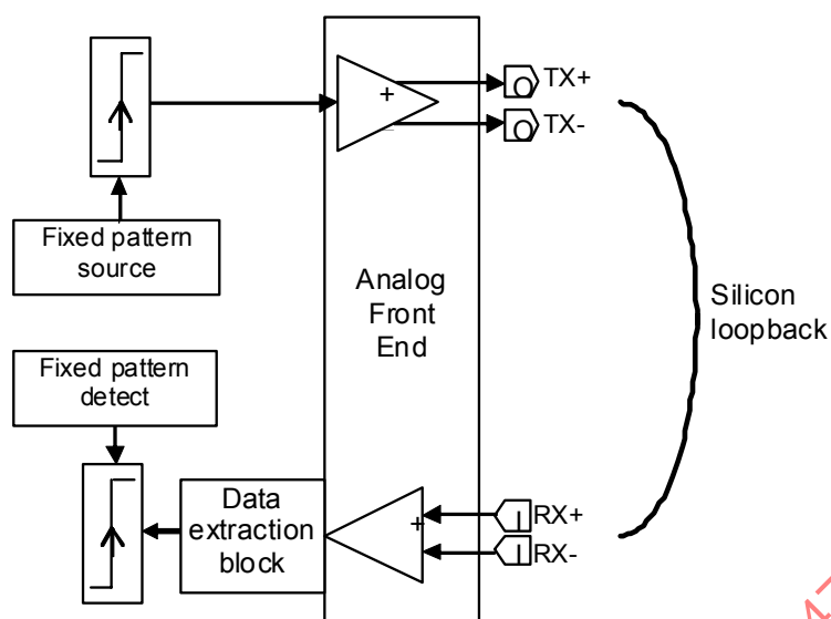
Figure 48 – Loopback, near-end analog
