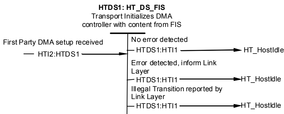
Figure 79 – Host transport decompose First Party DMA Setup FIS state diagram (State HTDS1)
