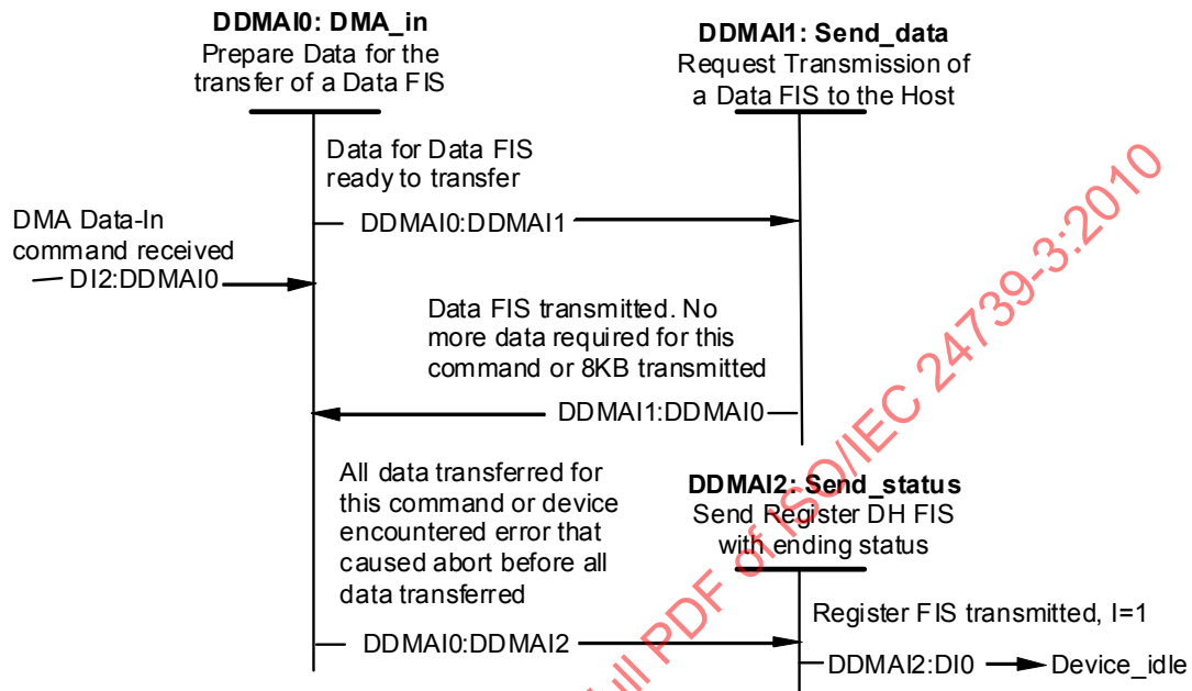
Figure 101 – DMA data-in command protocol (States DDMAI0-DDMAI1)
