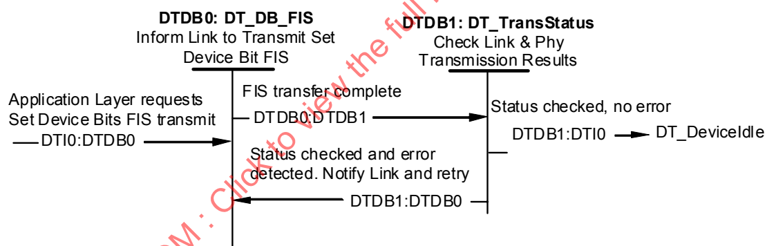
Figure 83 – Device transport send set device bits FIS state diagram (DTDB0-DTDB1)
