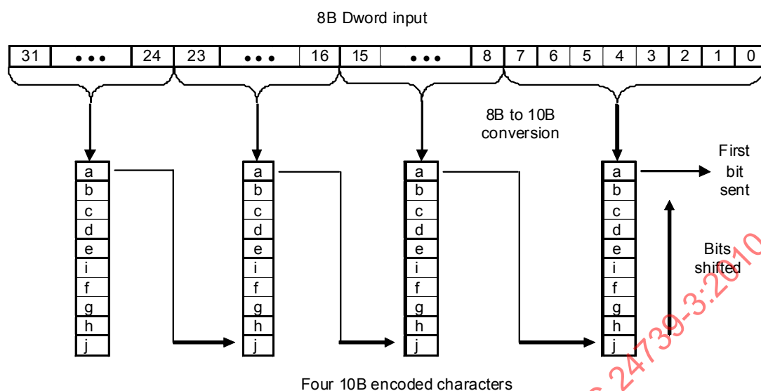
Figure 53 – Bit ordering and significance
