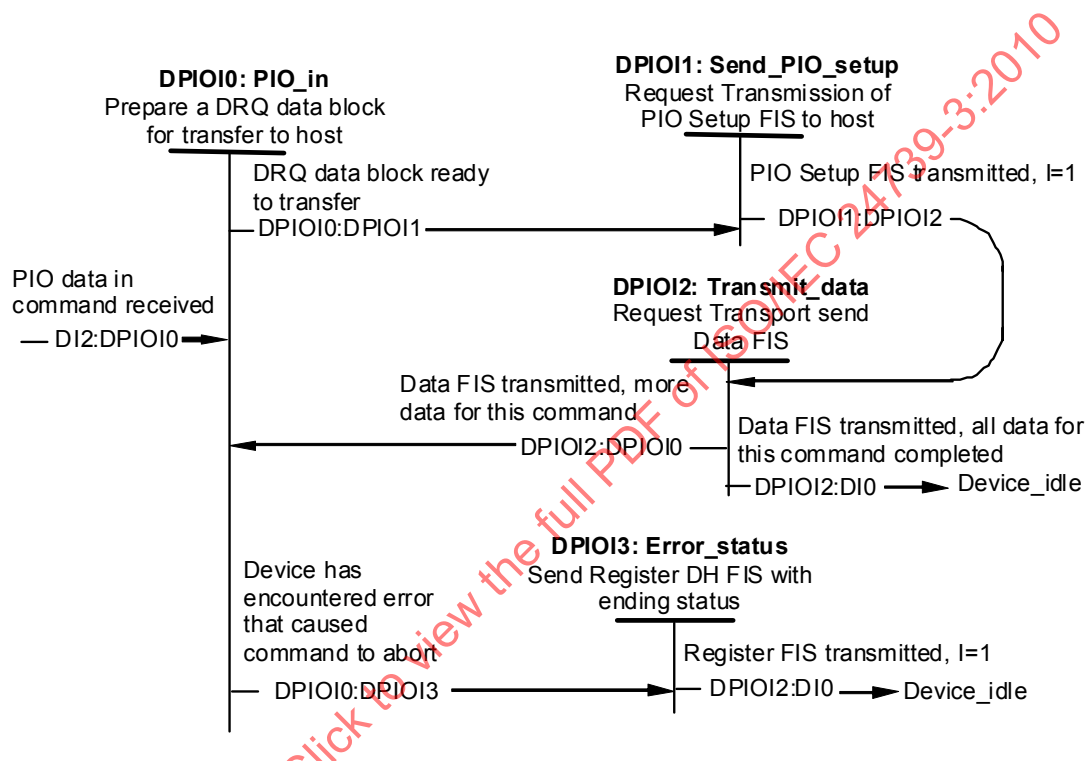
Figure 99 – PIO data-in command protocol (States DPIOI0-DPIOI3)
