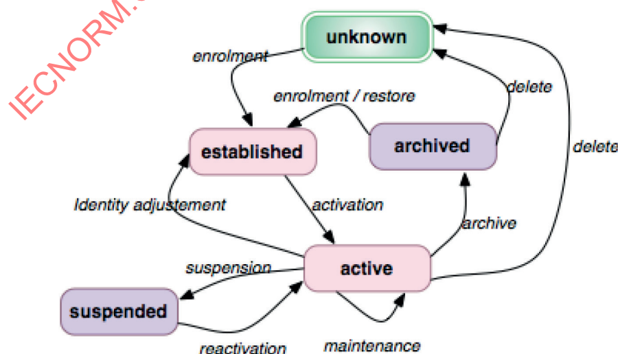
Figure 1 — Identity lifecycle
