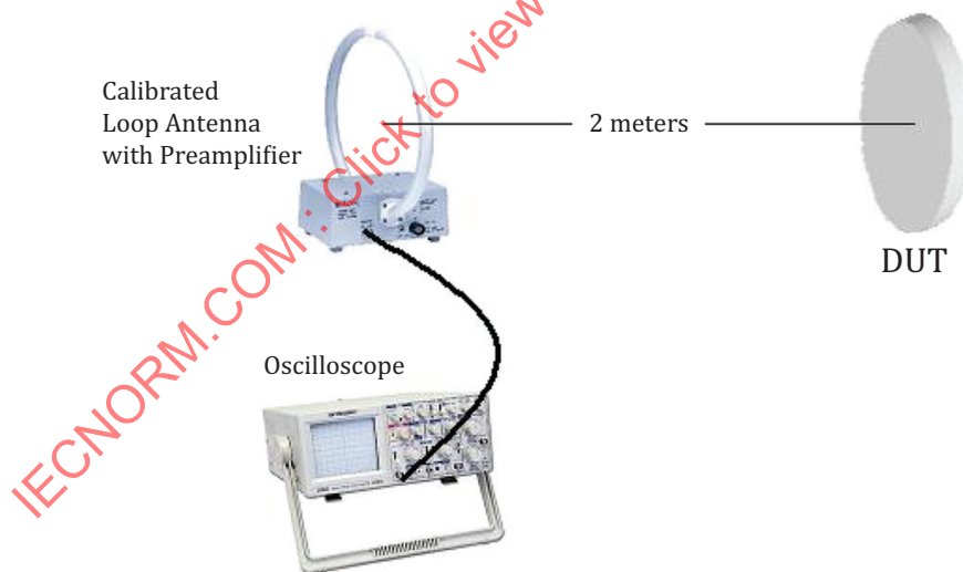
Figure 5 — Setup of equipment for exciter magnetic transmitter test
