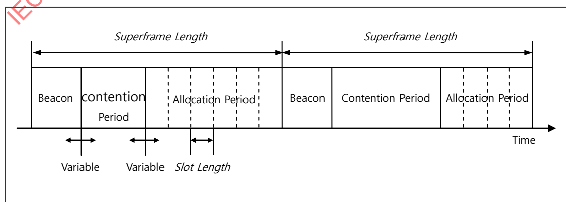
Figure 71 - Superframe synchronization
