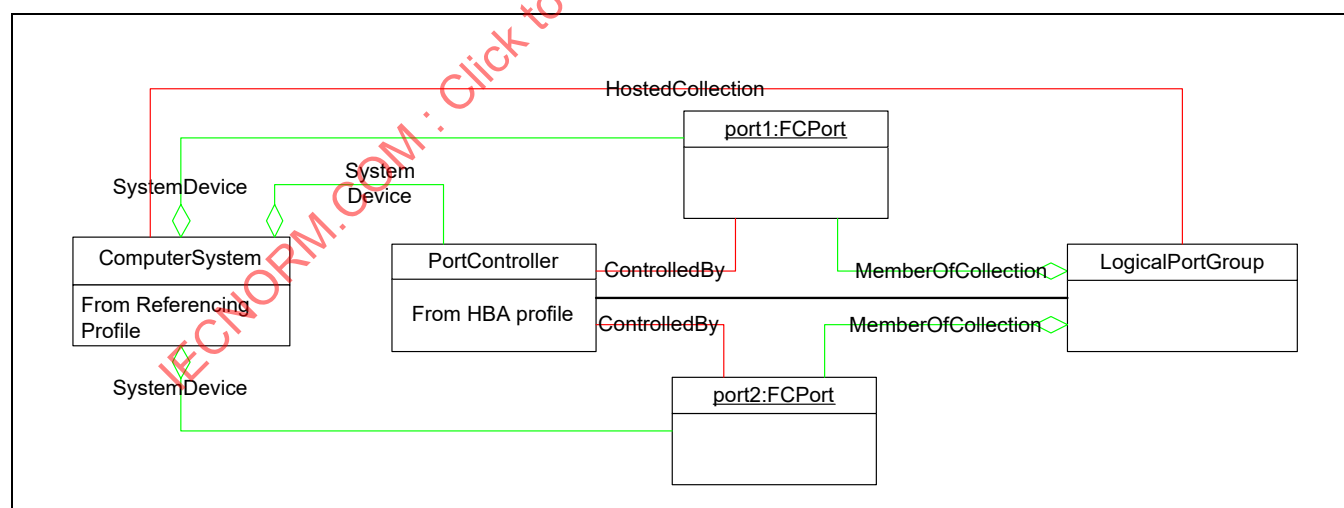
Figure 27 - FC Node Model
