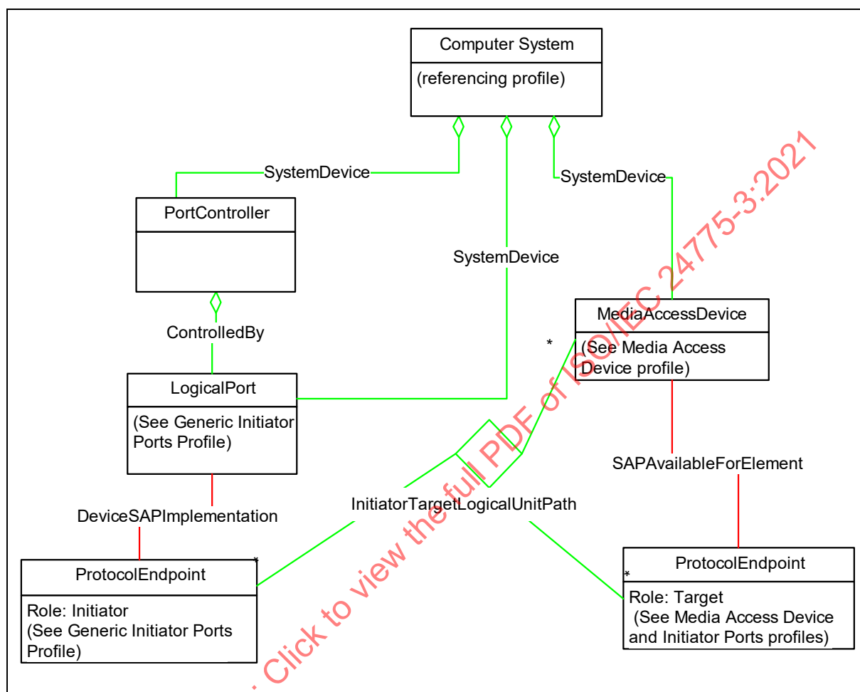
Figure 21 - HBA and Tape or Optical Devices
