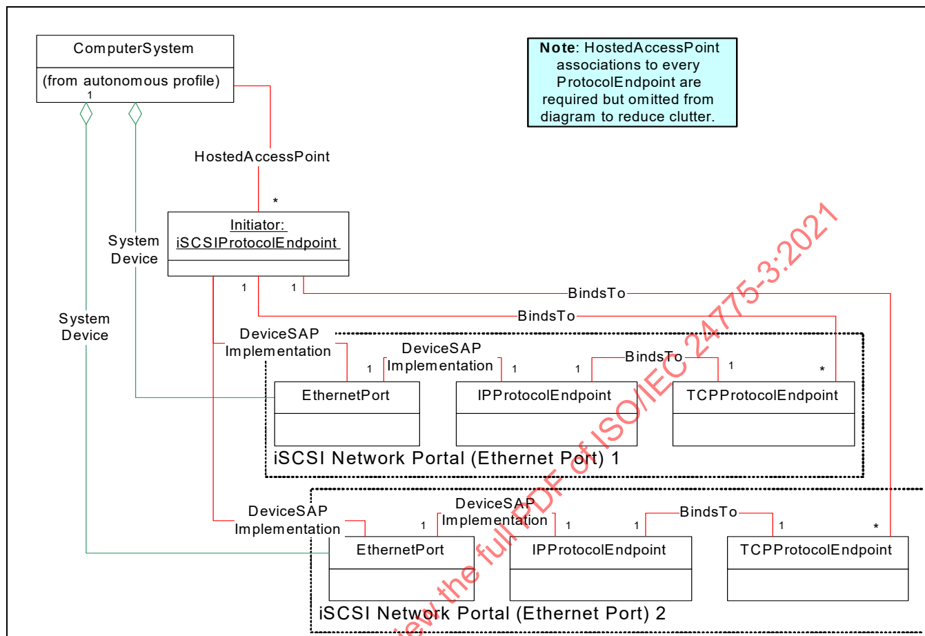
Figure 25 - iSCSI Initiator Port Instance Diagram
