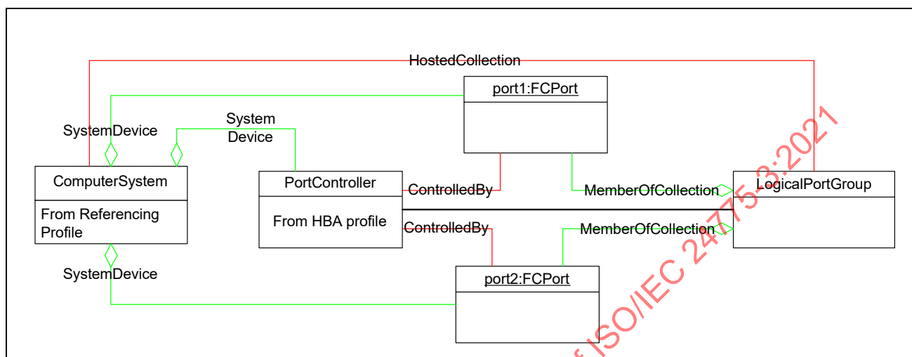
Figure 32 - Logical Port Group Model
