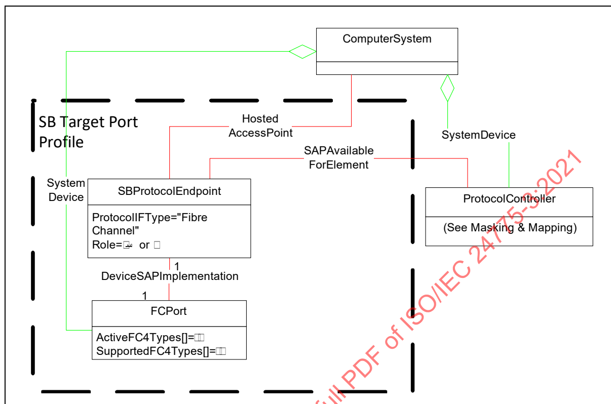
Figure 15 - SB Target Port Instance Diagram
