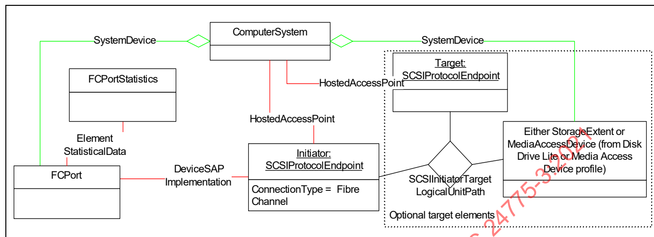
Figure 26 - Fibre Channel Initiator Instance Diagram
