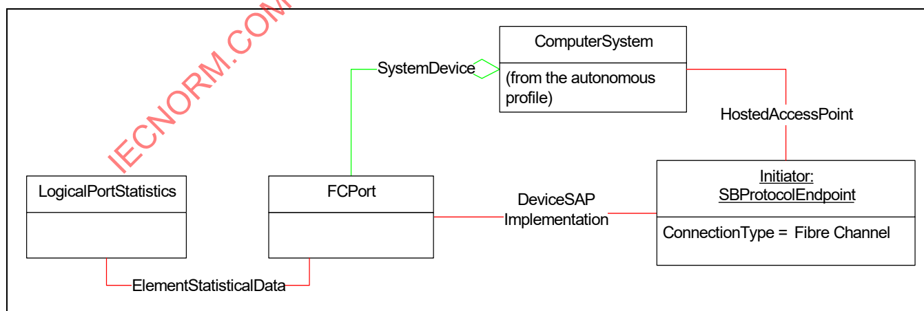
Figure 29 - Fibre Channel Initiator Instance Diagram
