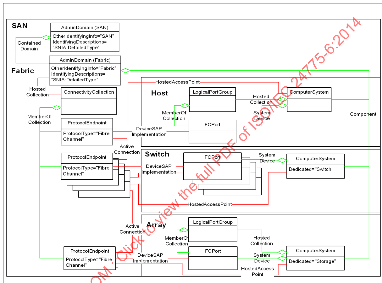
Figure 5 - Fabric Instance
