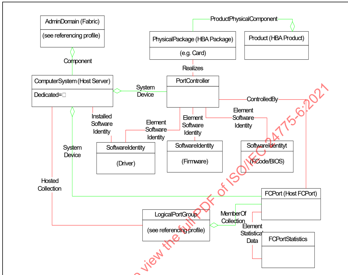
Figure 12 - FDMI Instance
