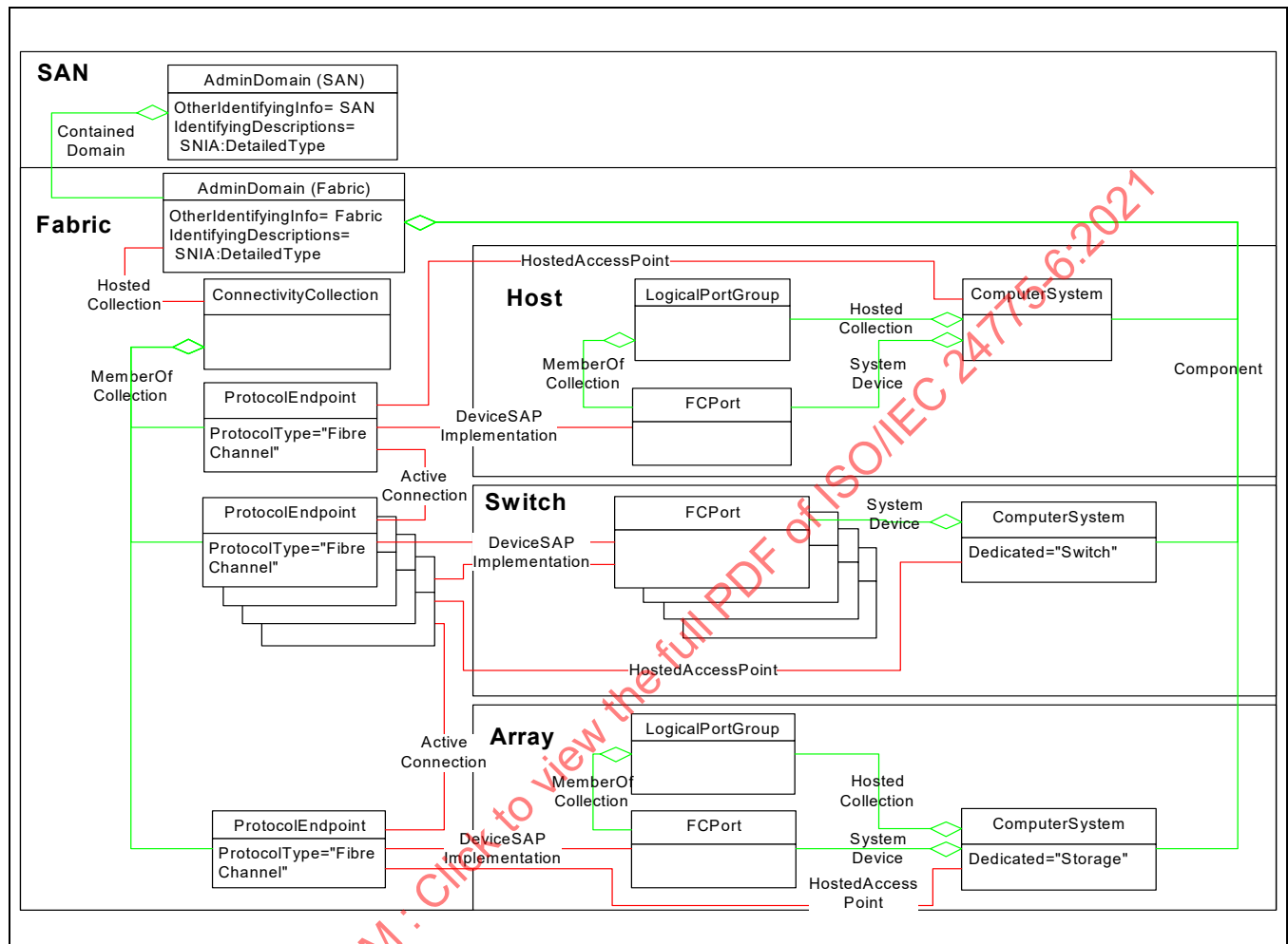
Figure 7 - Fabric Instance
