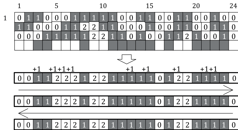
Figure C.5 — Steps and results of scanning row 4
