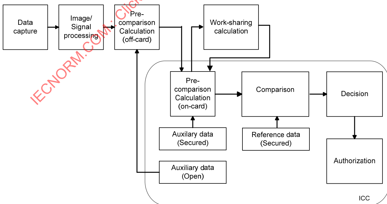
Figure 3 — General architecture for biometric authentication using work-sharing
