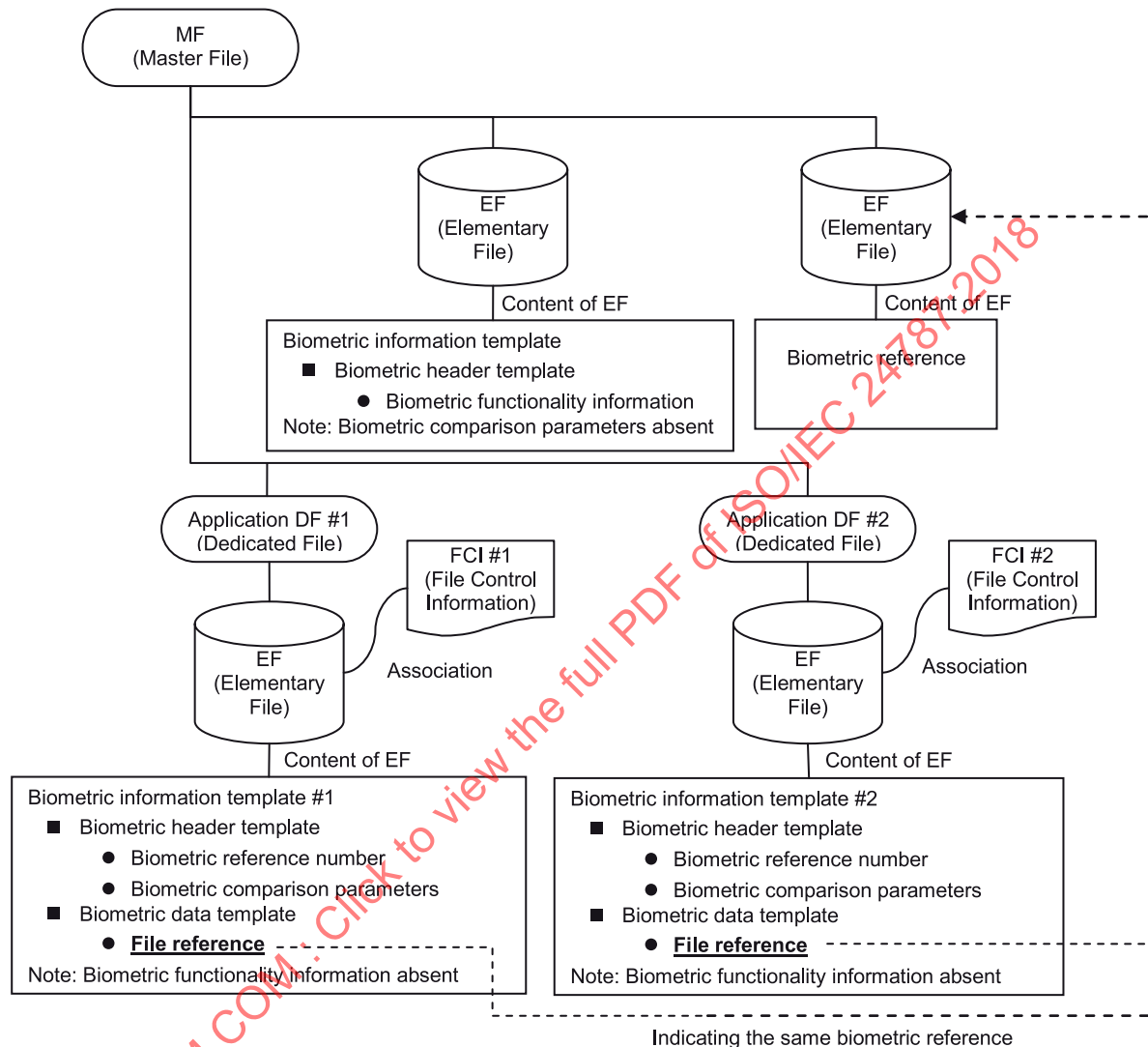
Figure B.1 — Example of file structure of one biometric reference for two applications
