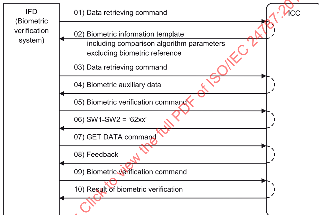
Figure 5 — Command-response APDU exchange for the work-sharing procedure
